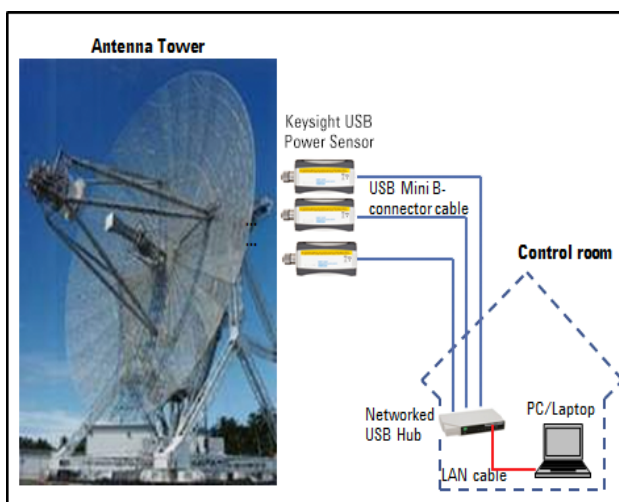
Figure 3. Multi-channel measurements via networked USB hub for antenna measurement simultaneously
