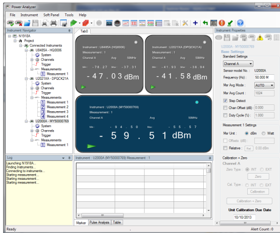
Figure 5. Power Analyzer (paid version license) support multiple power measurement display (max 4 display) at once and also offer additional features on top of Power Panel software
