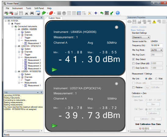
Figure 4. Power Panel (free version) software allow to support 2 USB power sensors measurement display only at once. Multilist view features offer in this version support multiple (more than 2) USB power sensors measurements.
