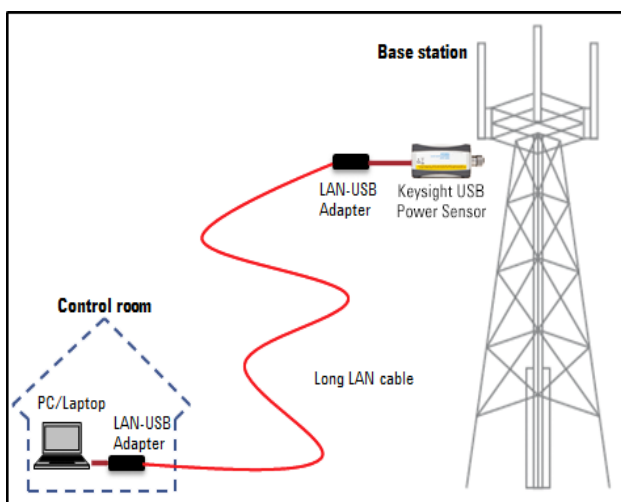
Figure 2. Single channel power measurement of USB power sensor using LAN-USB extender to extend the measurement distance for base station antenna application
