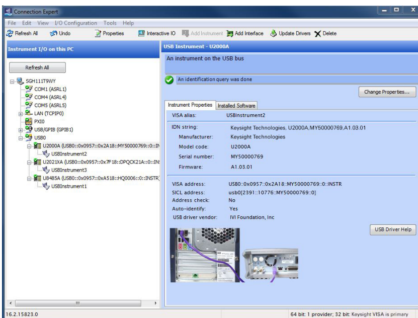
Figure 10. Keysight USB power sensors connectivity support auto-detected by Keysight IO Libraries Suite
