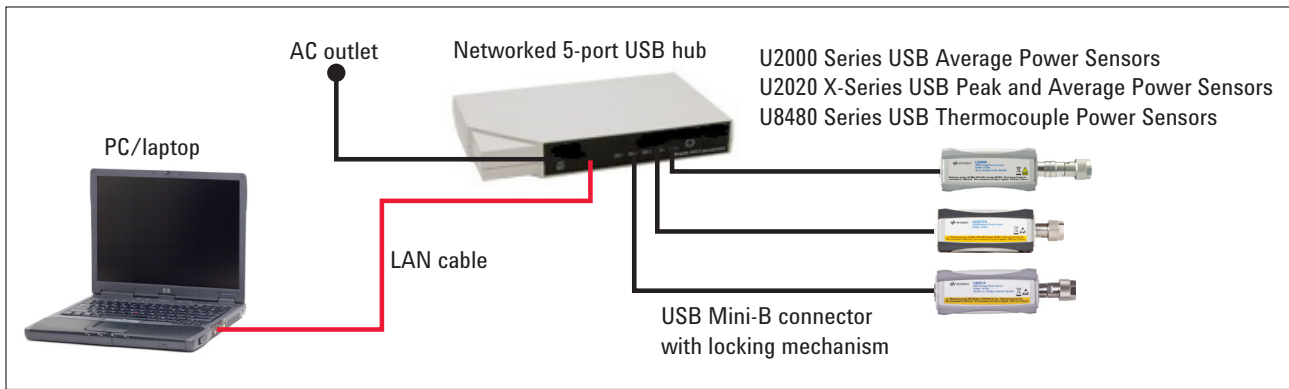
Figure 7. Keysight USB power sensors and networked 5-port hub setup diagram
