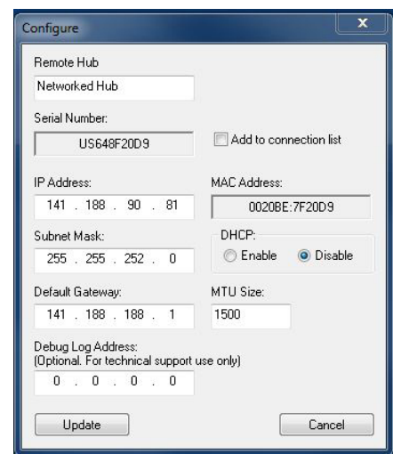
Figure 9. Configuring IP address, subnet mask, and default gateway in the networked hub configuration utility
