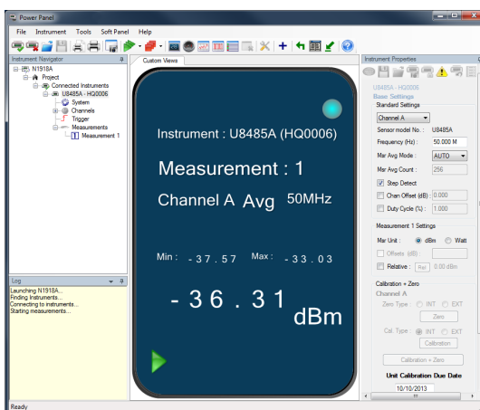
Figure 15. Single-channel power measurement via Keysight N1918A Power Analysis Manager, Power Panel software
