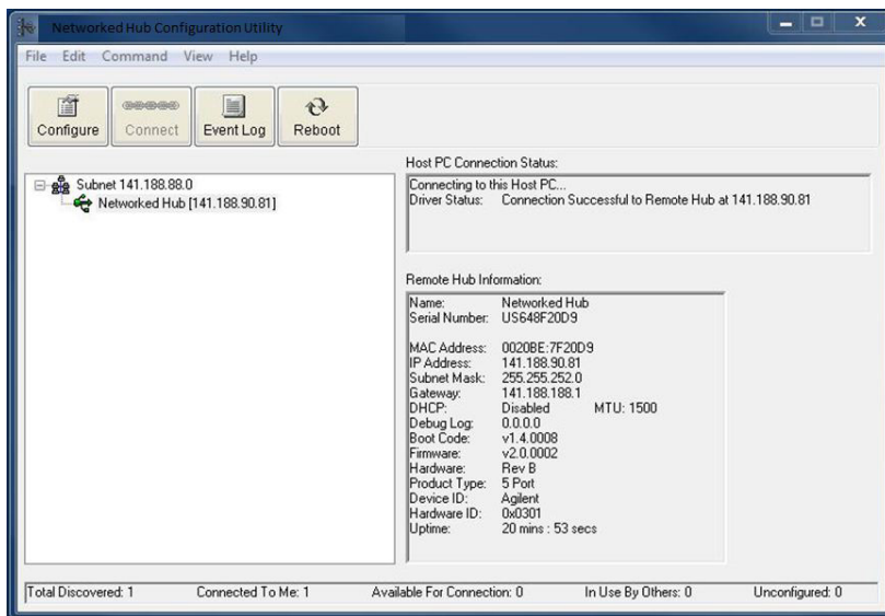
Figure 8. Networked Hub configuration utility display
