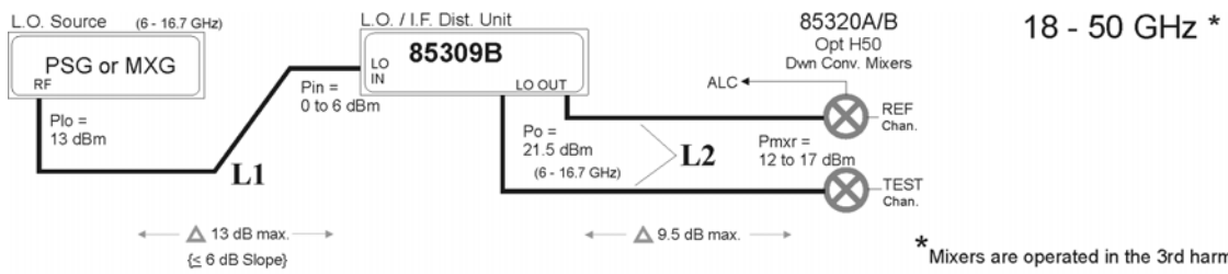
Figure 2-7 Cable Length configurations (2 of 2)
