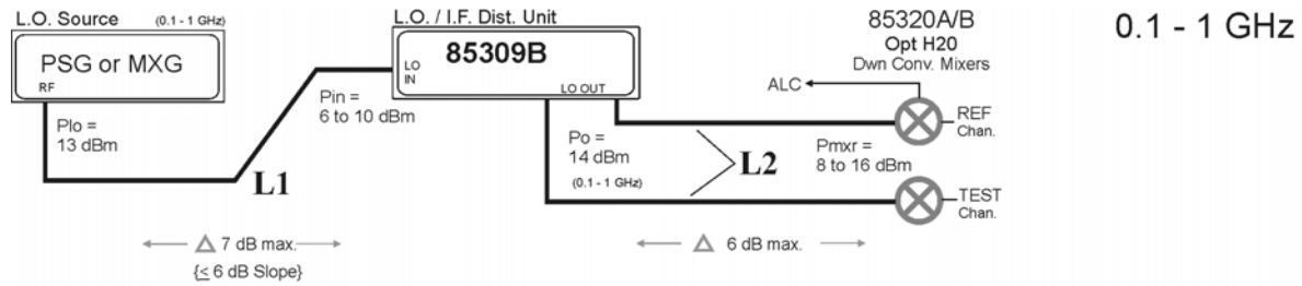
Figure 2-6 Cable Length Configurations (1 of 2)
