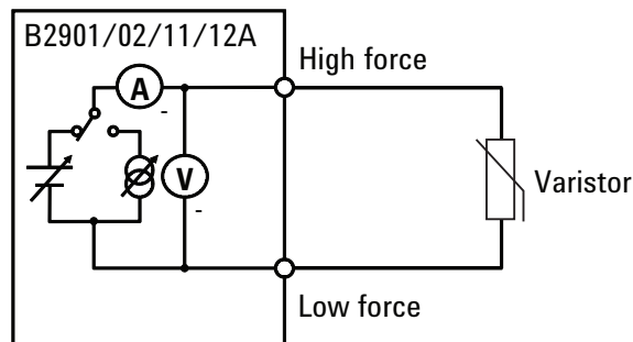
Figure 1. Image of the B2900A Series of SMUs and its circuit diagram to characterize a varistor
