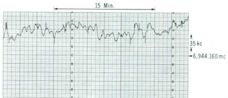
Fig. 5. Typical curve of drift measured in 6 mc oscillator with arrangement of Fig. 2. See also Fig. 3.
