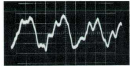
Fig. 3. Oscillogram of residual f-m in a 10 kmc measured signal made using setup of Fig. 2. Vertical sensitivity is 25 kc/division. Sweep time is 5 milliseconds/cm.
