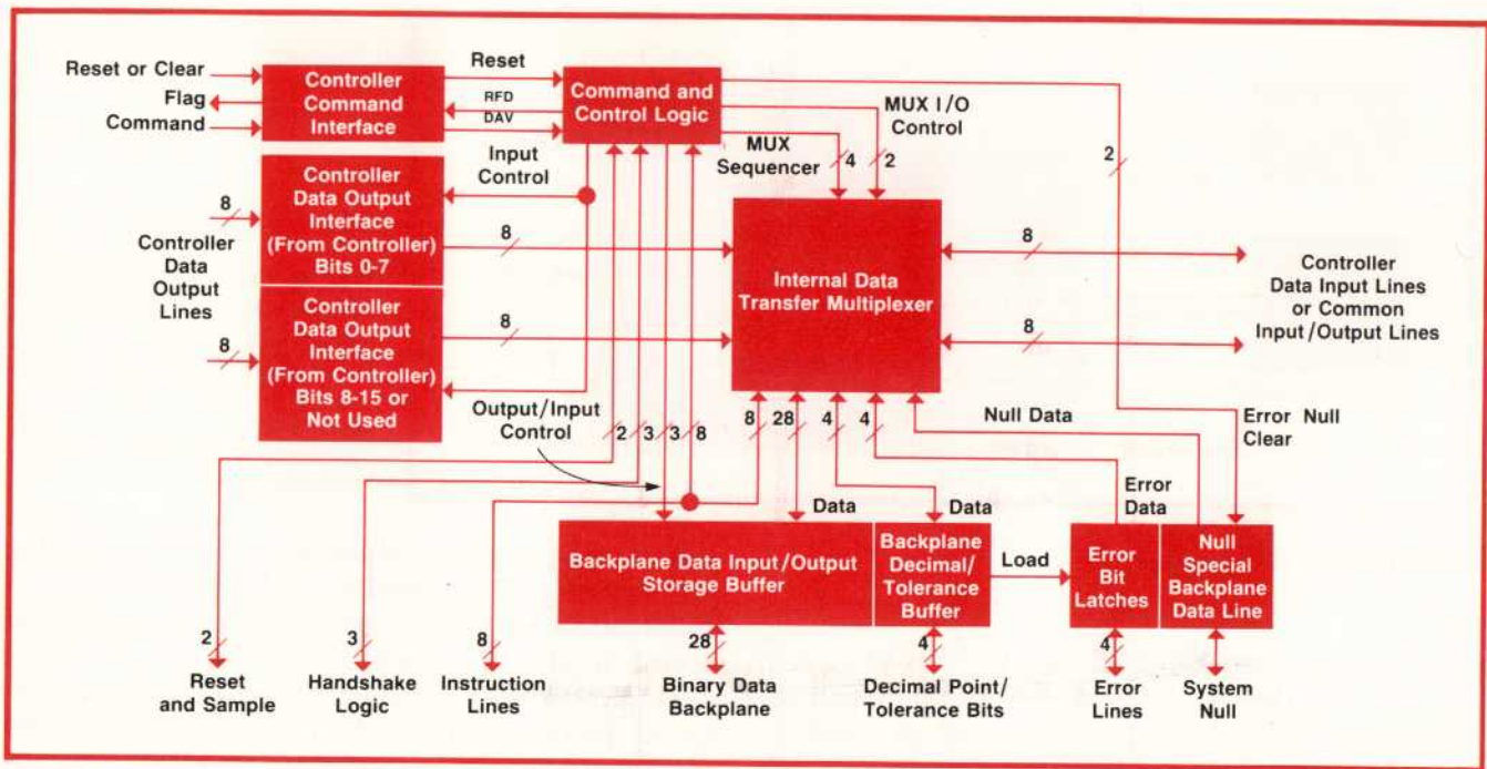
Fig. 5. The 10746A Binary Interface is an I/O card suitable for interfacing the laser transducer system to a variety of computers and digital controllers.
