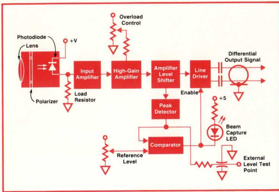
Fig. 3. 10780A Receivers, one for each measurement axis, convert the received laser light to electrical signals. Laser head and receiver enclosures meet NEMA-12 standards for industrial packages.
