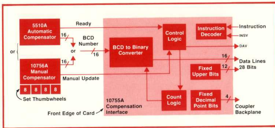
Fig. 4. The 10755A Compensation Interface card places an environmental velocity-of-light compensation factor on the coupler backplane. It gets this factor from the 5510A Automatic Compensator or from the 10756A Manual Compensator.
