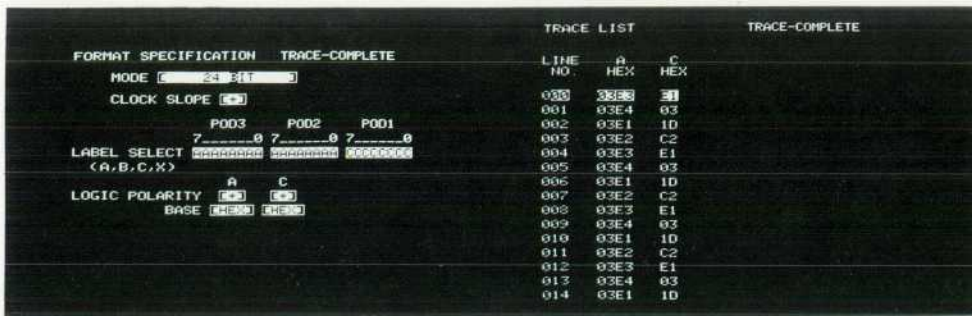
Fig. 3 When configured as a 24-bit logic state analyzer, Model 1615A allows the user to label the input probes and select the numerical base for the captured data, using the FORMAT SPECIFICATION "menu" (left), for easier interpretation of the captured data when displayed on the TRACE LIST (right).
