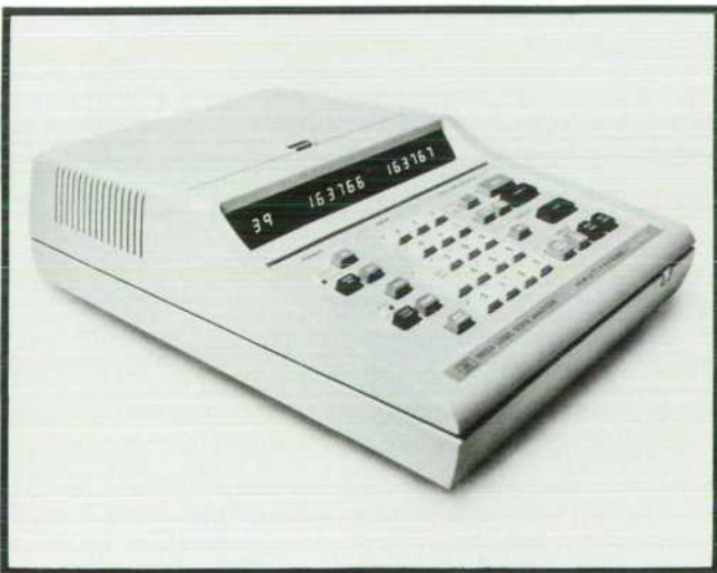
Fig. 1. Model 1602A Logic State Analyzer captures and stores for analysis sequences of 64 digital words up to 16 bits wide occurring at rates up to 10 MHz. Although designed for ease of use, it is capable of seeking and capturing the desired information in complicated programs.
