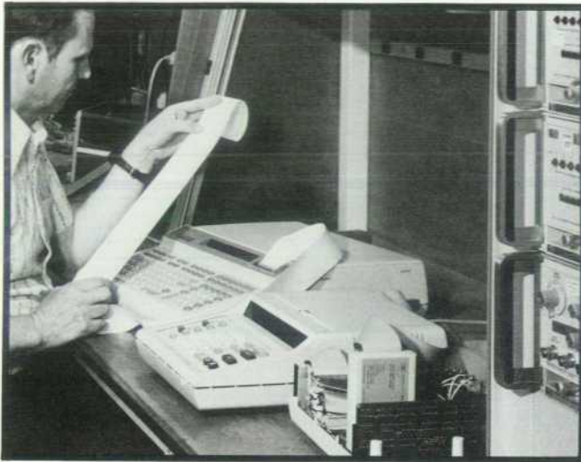
Fig. 5. Model 1602A, shown here with a Model 9825A Desktop Computer, is programmable by way of the HP Interface Bus and is thus easily adapted to automatic test systems.
