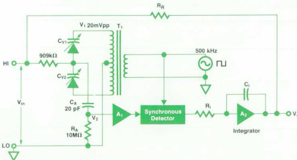
Fig. 9. The input amplifier used in the 4140A has a high dc input impedance since there is no dc path in the input circuit. In the absence of an input, the bridge formed by transformer T_1 and capacitances C_{v1} and C_{v2} is balanced. An input voltage unbalances C_{v1} and C_{v2} differentially and an ac voltage, V_2 , then appears at the input to amplifier A_1 .
