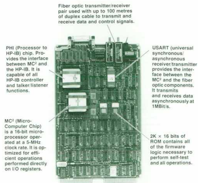
Fig. 4. The fiber optic link has a single printed circuit board with a combination of advanced technologies.
