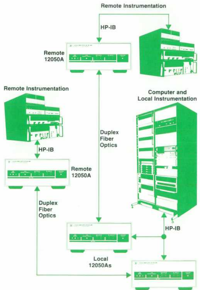
Fig. 3. The fiber optic link makes it easy to duplicate a group of HP-IB instruments at several sites, using a single computer at one site (many production test stations are in this category).
