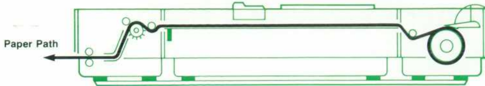
Fig. 2. Paper drive system holds the paper flat against the platen by applying constant tension to the paper web.
