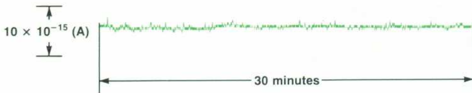
Fig. 10. Recording demonstrates the stability of the 4140A on its most sensitive range. For this test, the source resistance was 100 G \Omega and the measurement integration time was set to LONG.
