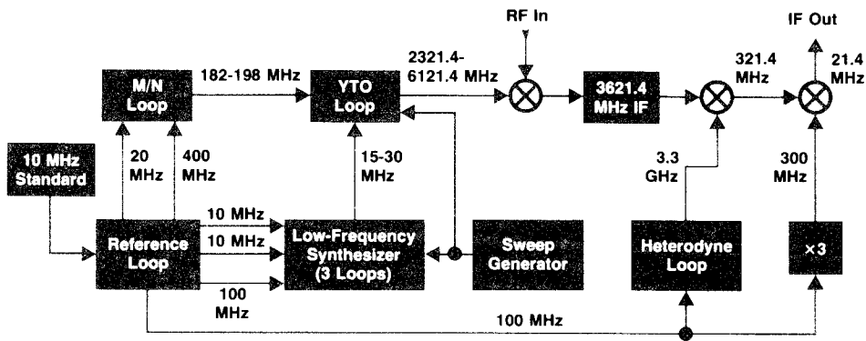
Fig. 1. Frequency conversion chain uses seven phase-locked loops, two of which can be swept. All are referenced to a 10-MHz oven-controlled crystal frequency standard that has an aging rate of less than one part in 10^9 per day.
