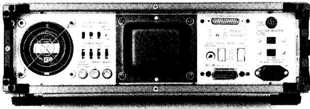
Fig. 8. The ENABLE SELECT switches and two of the four ENABLE inputs are on the rear panel. Also on the rear panel are the LOGIC POLARITY switches, DAV DELAY adjustment, RS232C BAUD RATE select, and HP-IB addresses (KEYBOARD and DATA MODES).
