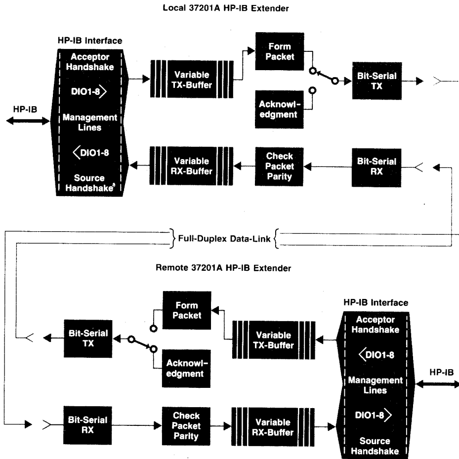
Fig. 3. Simplified block diagram illustrates the functional operation of a pair of 37201A HP-IB Extenders.
