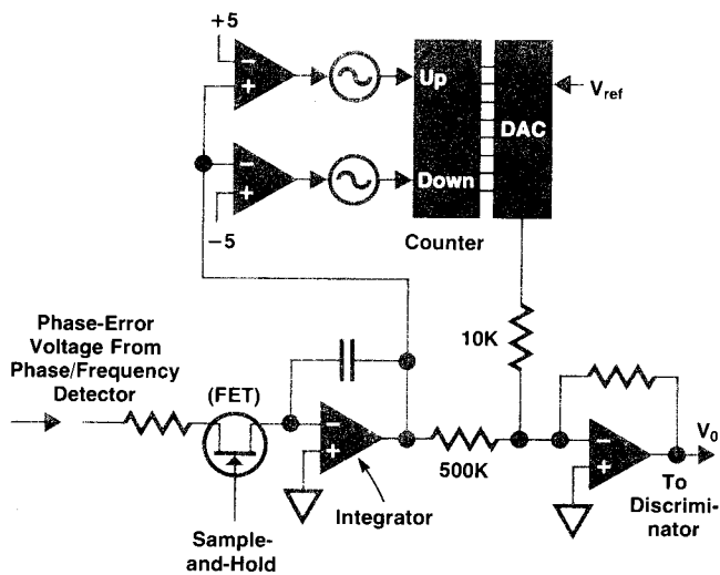
Fig. 2. Digital sample-and-hold.
