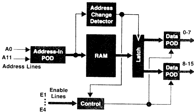
Fig. 6. Block diagram of the Model 8170A Logic Pattern Generator operating in the external address mode. Data is output whenever the address-change detector, consisting of exclusive-NOR gates, detects that there has been a change of address. Alternatively, one of the enable inputs may be used as a clock input for timing the data output. A data-valid signal is also generated.
