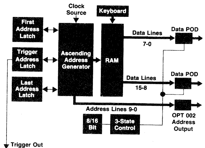
Fig. 3. Block diagram of the 8170A operating in the internal address mode. In this mode, the memory contents are supplied to the outputs in ascending order beginning at the first address specified and ending at the last address. A trigger output pulse is generated whenever the address being accessed in memory matches the address in the trigger address latch.
