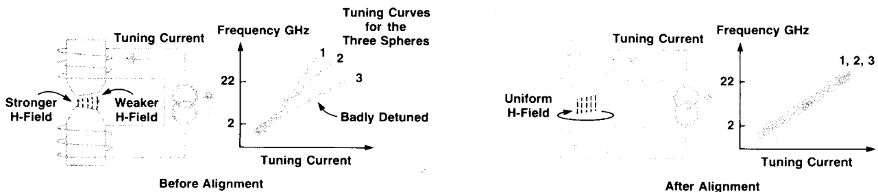
Fig. 3. Misalignment of the tuning magnet pole faces, shown exaggerated here, causes the three YIG spheres to have different tuning characteristics. Rotating the tilted faces into parallel alignment achieves identical tuning characteristics for the three spheres.
