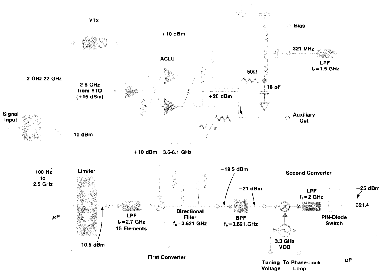
Fig. 1. Block diagram of the input section of the Model 8566A Spectrum Analyzer. The control microprocessor selects the appropriate signal path according to the frequency span selected.
