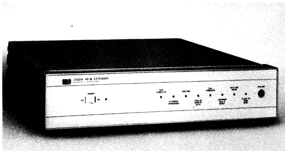
Fig. 1. The Hewlett-Packard Model 37201A HP-IB Extender converts standard HP Interface Bus activity into a serial form for communication via normal full-duplex modems or twin-pair cable. Functioning in pairs, extenders enable two distant clusters of bus-interfaced instruments to operate as one.
