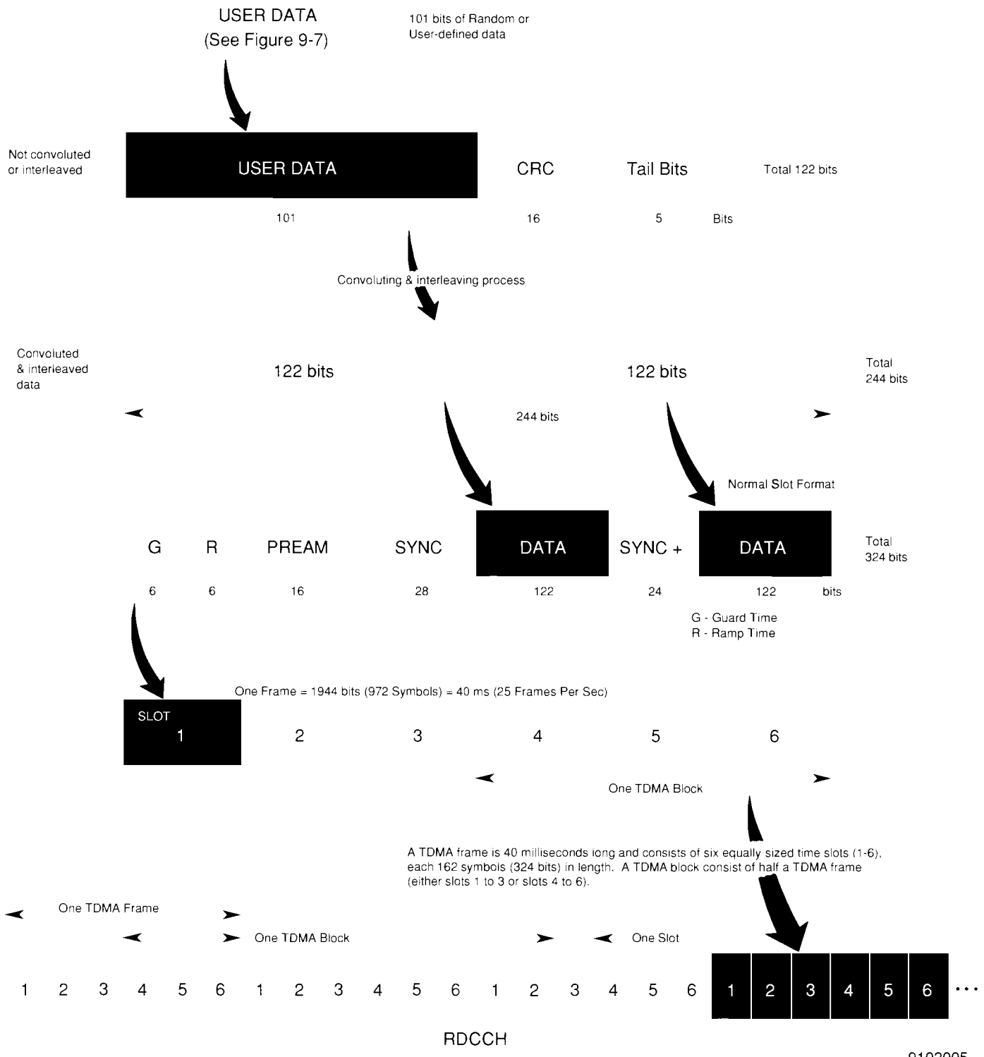
Figure 9-4 Normal Length Message in the RDCCH
