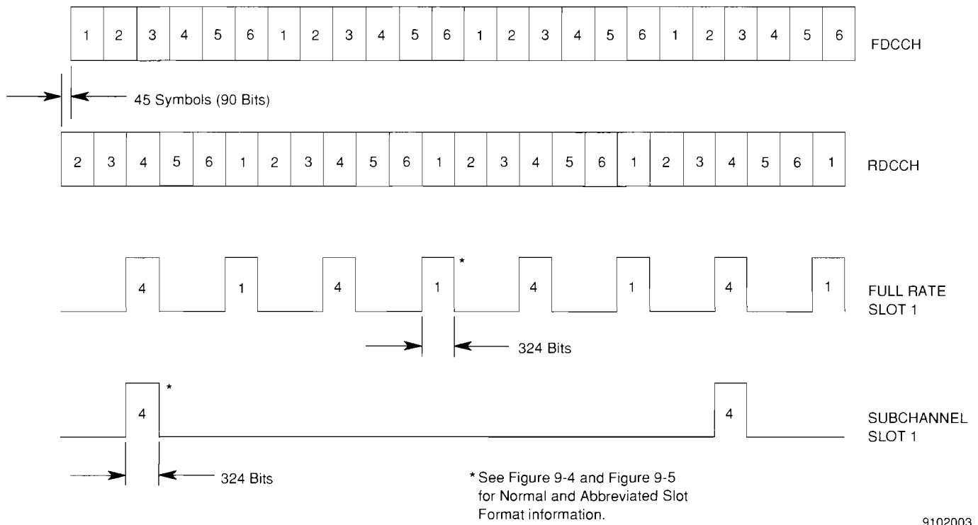
Figure 9-6 Contiguous and Sub Channel Transmissions
