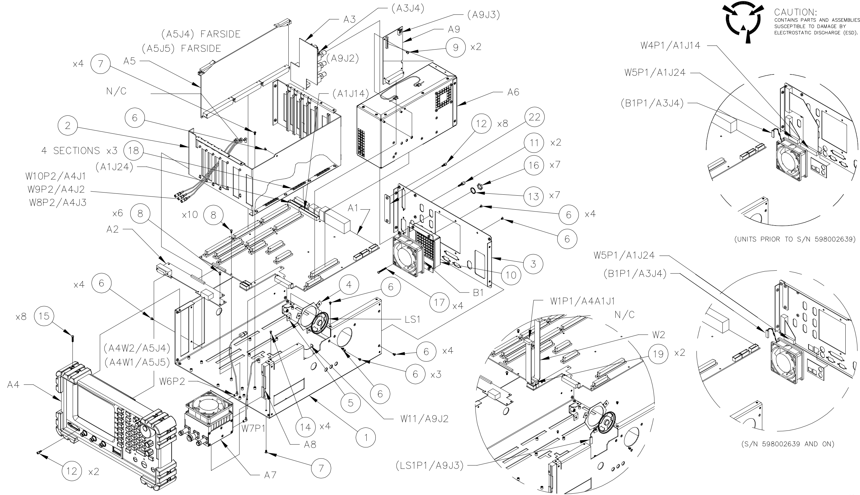
Figure 4-3 2975 Chassis Assy
