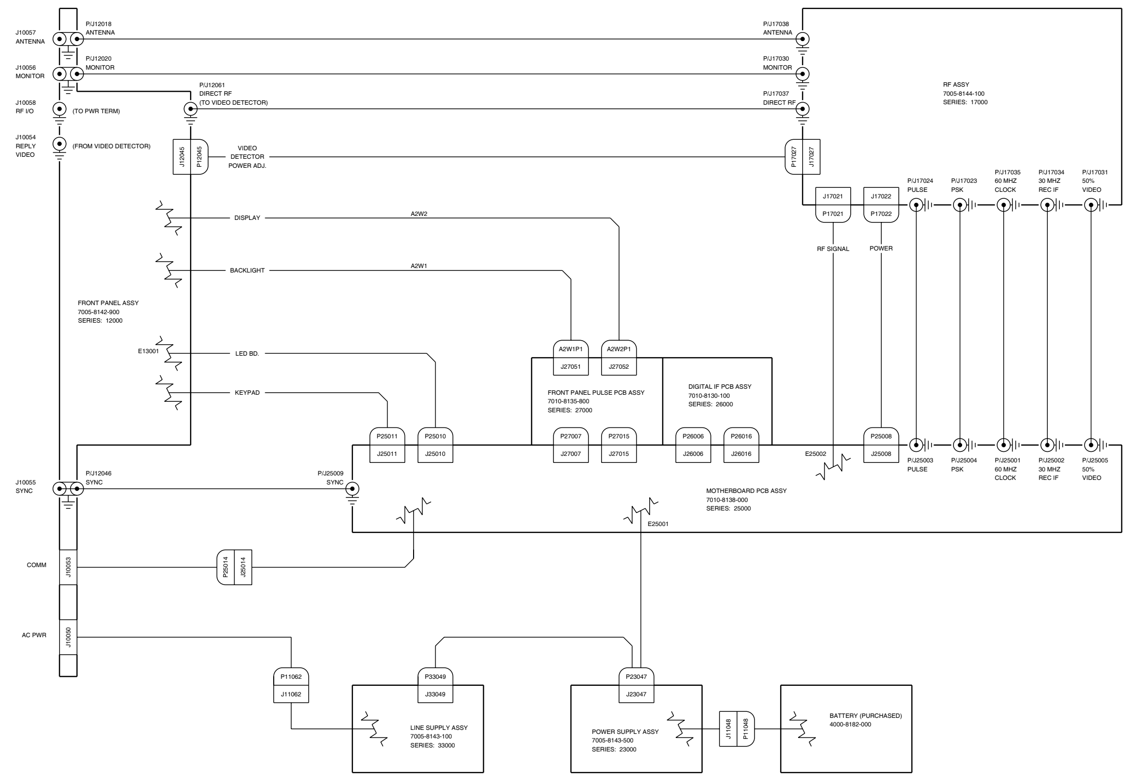
Composite Assembly Interconnect Diagram (0000-8145-300-C)
