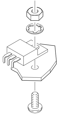
DETAIL B
