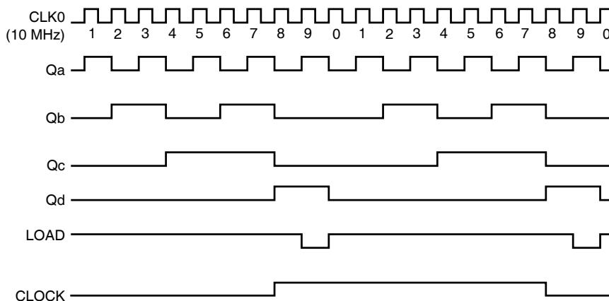
500 kHz Clock Timing Diagram Figure 6
