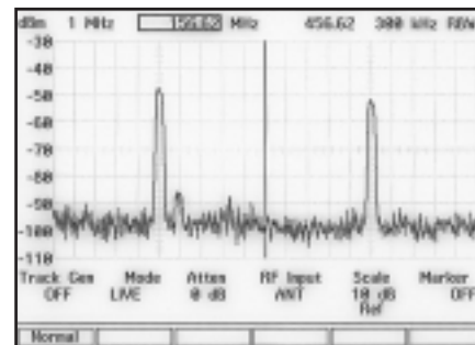
Split screen spectrum analyzer gives you more flexibility
