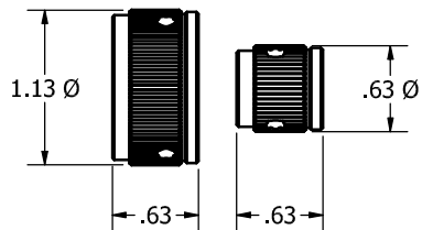
KNOB DETAIL
