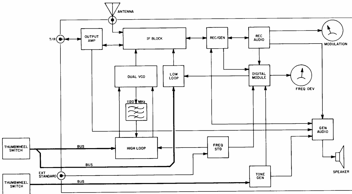
Figure 2-2 Simplified Block Diagram
