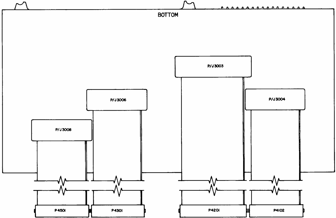
Figure 9-1 Motherboard PC Board Assembly (3000)
