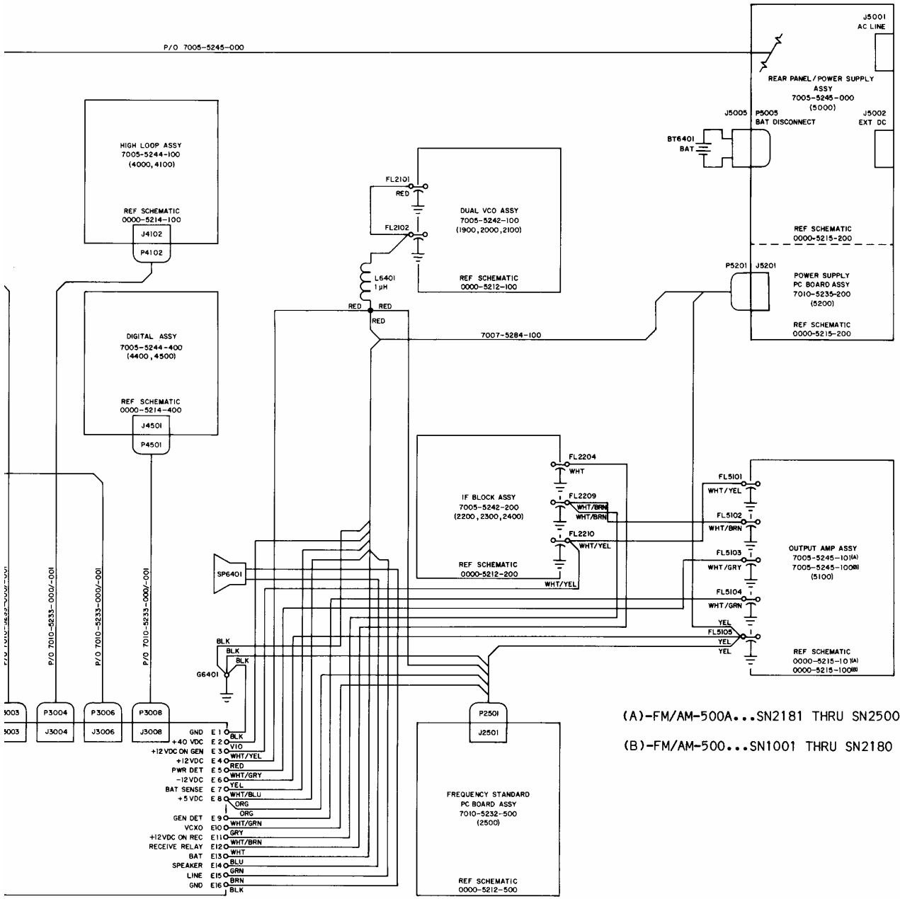
Figure 10-2 Electrical Interconnect (SN 1001 thru SN 2500)
