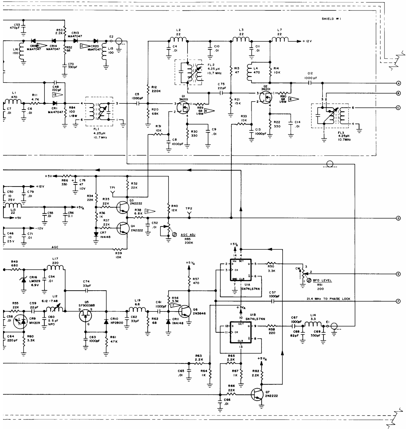
Figure 10-17 Receiver/Generator Module Circuit Schematic (Sheet 1 of 2)
