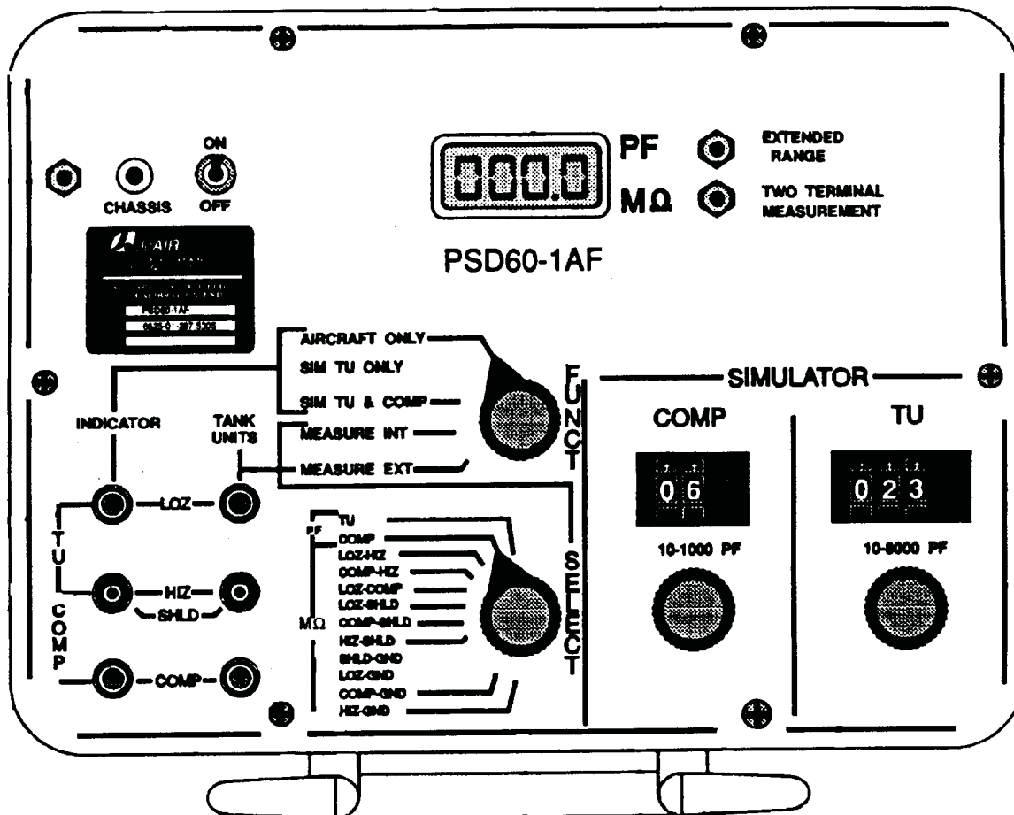
Figure 1. Front panel.
