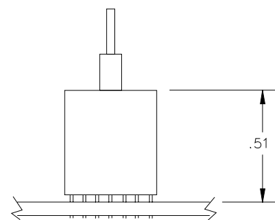
DETAIL "C"
