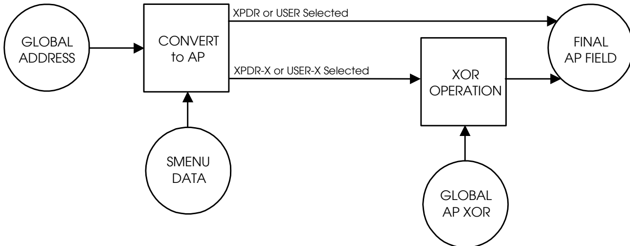
Sequence Menu Interrogation AP Field Formation Figure 38
