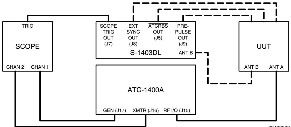
Mode S Test System Operational Hook-Up Diagram Figure 2
