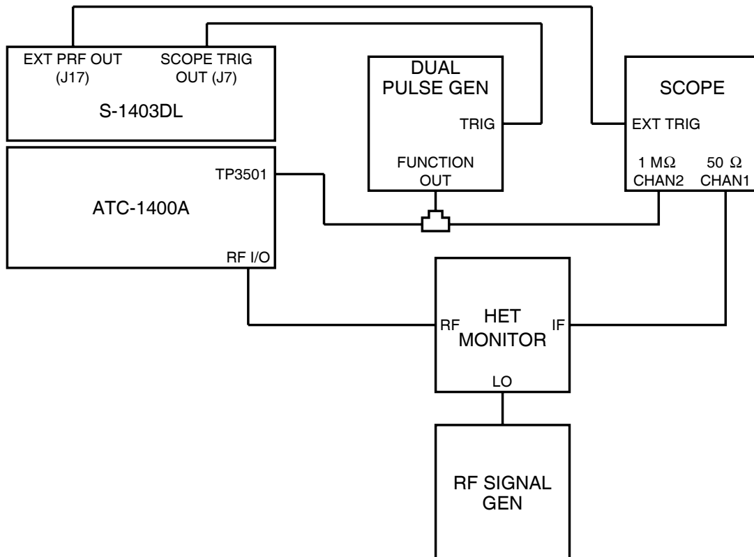
Installation Calibration Test Setup #3 Diagram Figure 4
