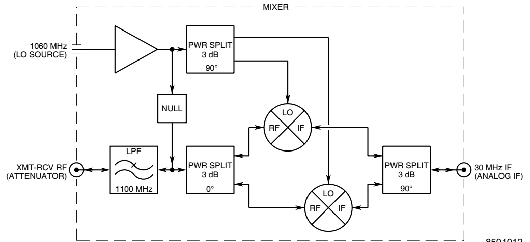
Mixer PCB Assy Block Diagram Figure 11
