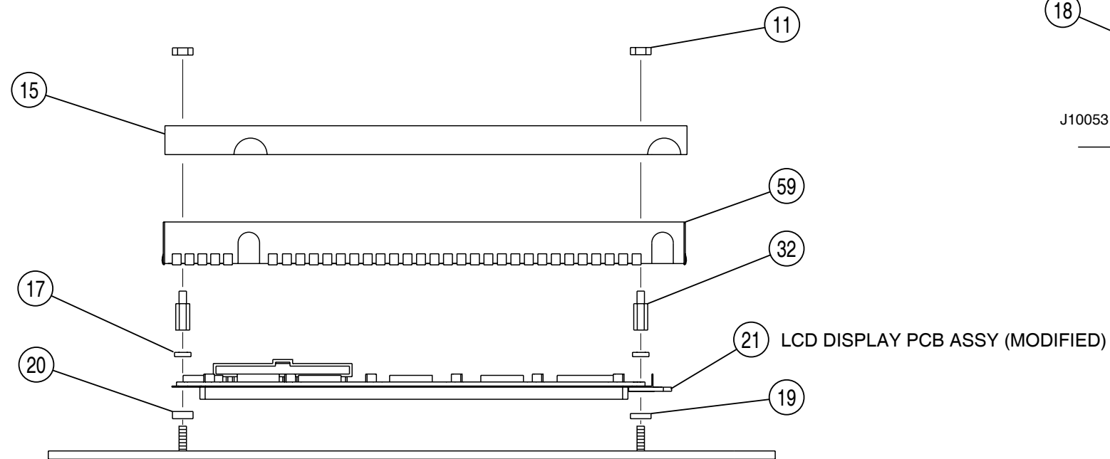
DETAIL A
