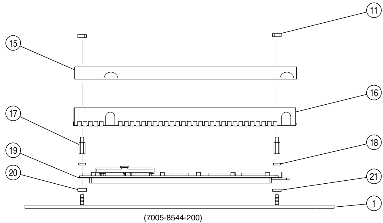
DETAIL B
