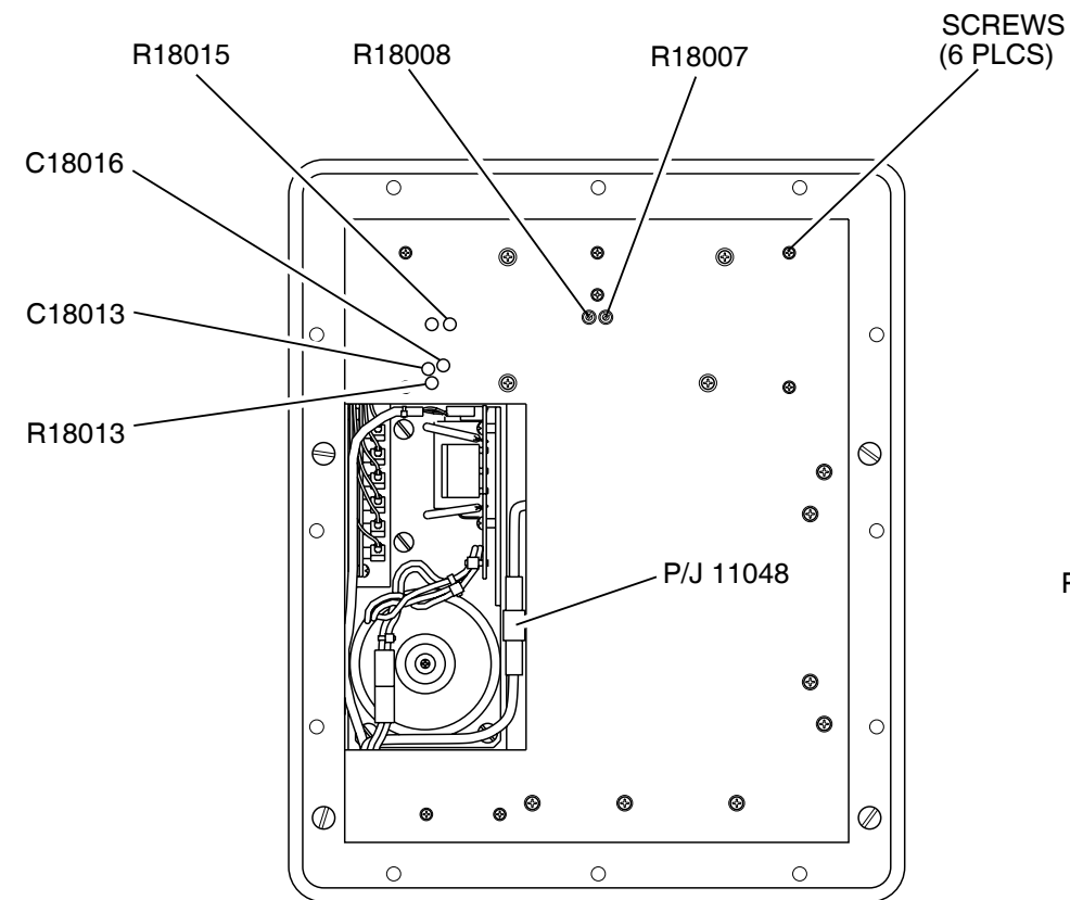
REAR VIEW
