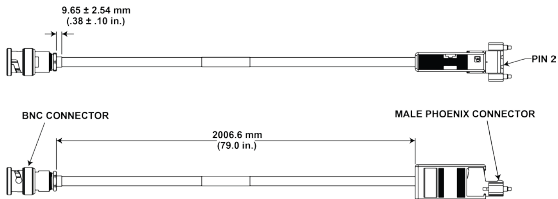
Figure 2: 8020-SHI-BNC-2 cable assembly dimensions
