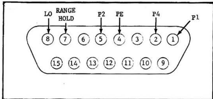
FIGURE 6. Remote Ranging Connector.
