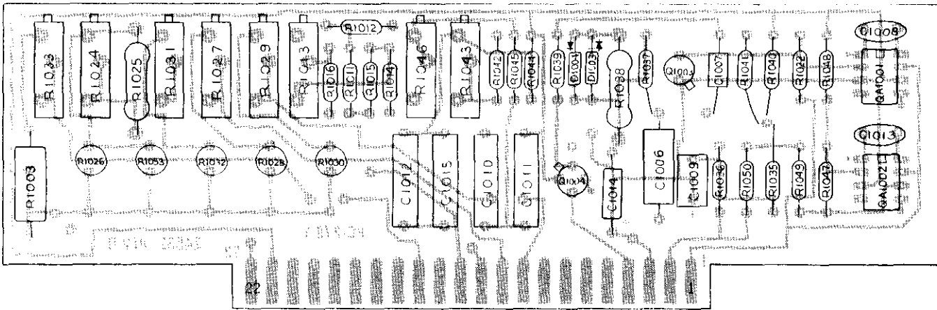
FIGURE 26. Component Layout, PC-279
