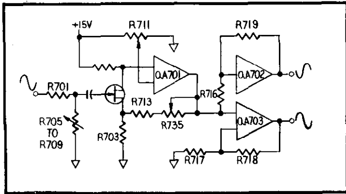
FIGURE 12. AC Amplifier, 2nd Stage.
