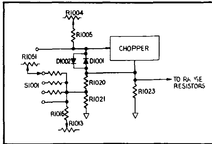
FIGURE 15. Zero Suppression Circuit
