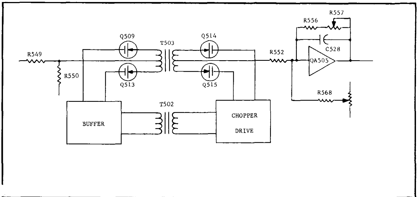
FIGURE 16. Isolator Circuit.
