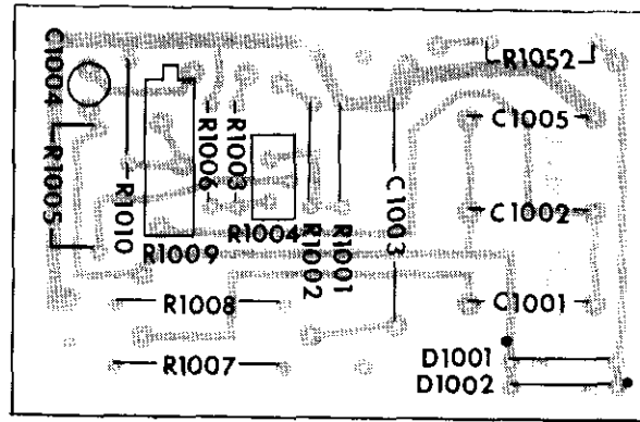
FIGURE 25. Component Layout, PC-278
