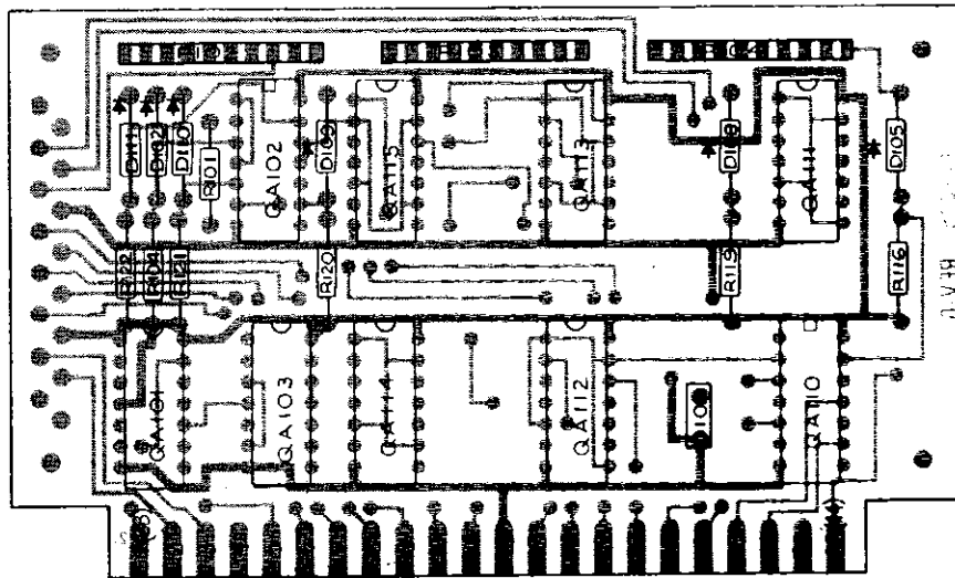
FIGURE 35. Component Layout, PC-275 (Part 1)
