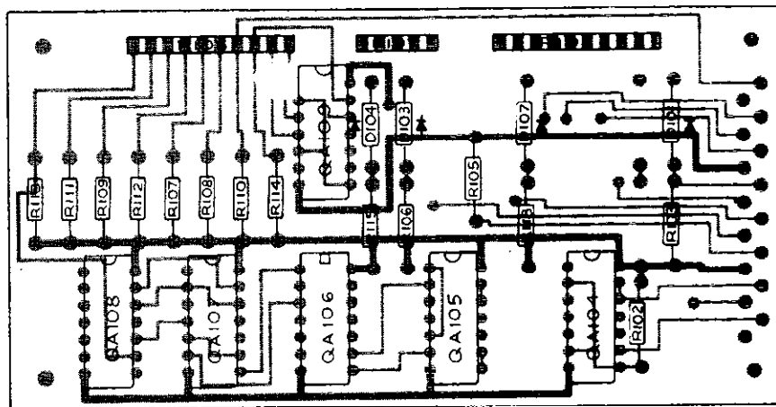
FIGURE 36. Component Layout, PC-275, (Part 2)
