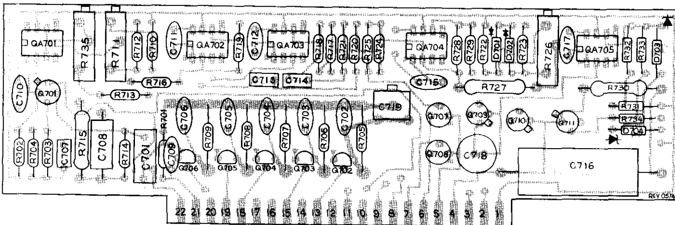
FIGURE 27. Component Layout, PC-282
