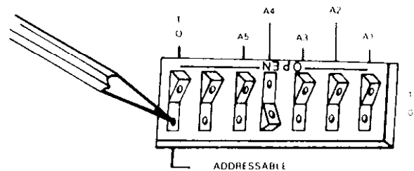
Figure 3-7. TO/ADDRESSABLE and Primary Address Switches (Address Eight Shown)
