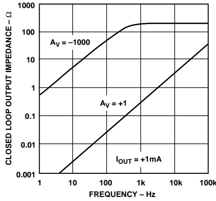
Figure 20. Magnitude of Closed Loop Output Impedance vs. Frequency
