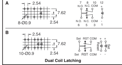
Fig. 2 DK Series - PCB
