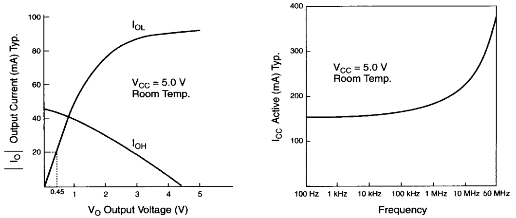
Figure 16. Typical Output Drive Characteristics & I_{CC} vs. Frequency
