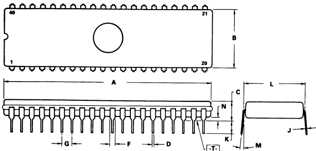
S SUFFIX CERDIP PACKAGE CASE 734A-01
