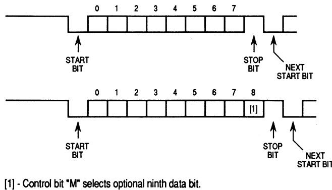
Figure 5-1. Data Format
