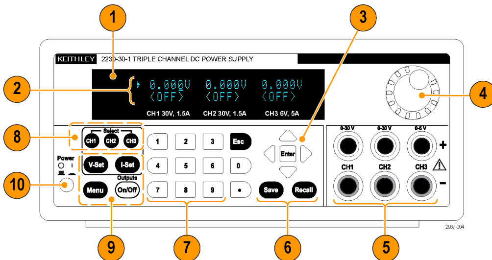
Figure 1: Front-panel of the model 2230-30-1, which has three output channels.
