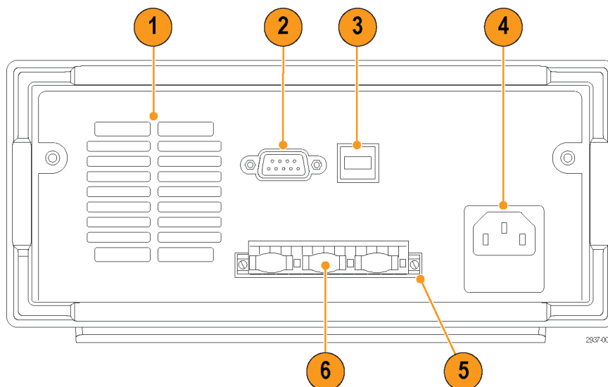
Figure 2: Rear-panel of the 2230-30-1.
