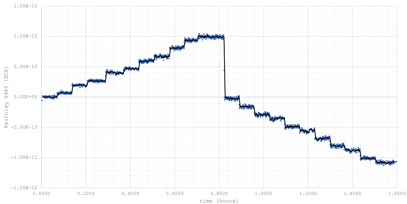
Keithley 238 Sensitivity
