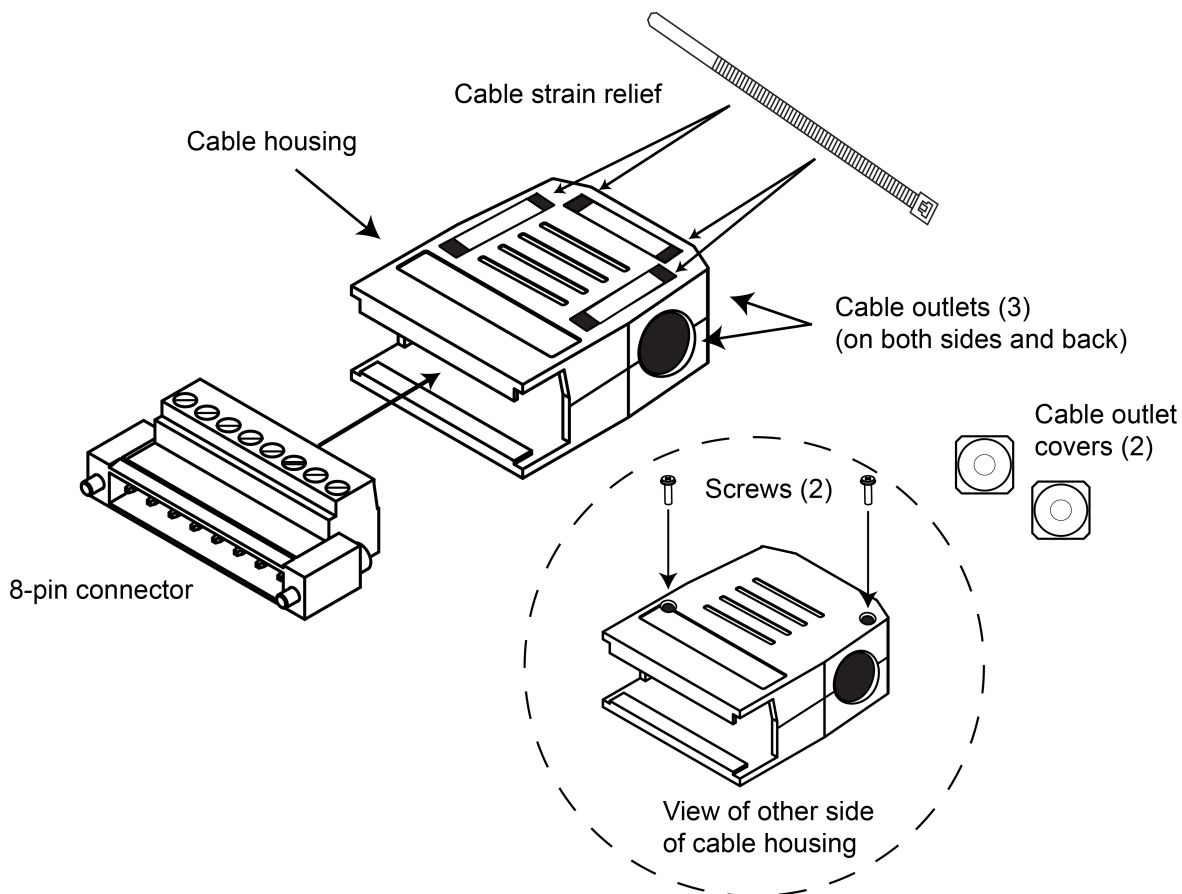
Figure 1: Model 2460-KIT
