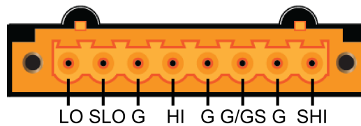
Figure 2: Model 2460 screw terminal pinouts
