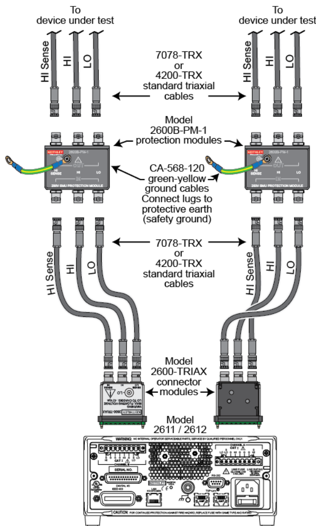
Figure 4: Model 2600B-PM-1 connections for Model 2611 or 2612
