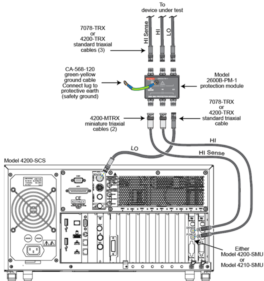
Figure 7: Model 2600B-PM-1 connections for Model 4200-SCS SMU
