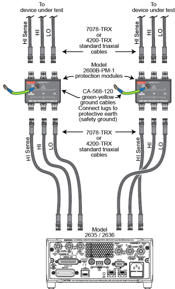
Figure 5: Model 2600B-PM-1 connections for Model 2635 or 2636
