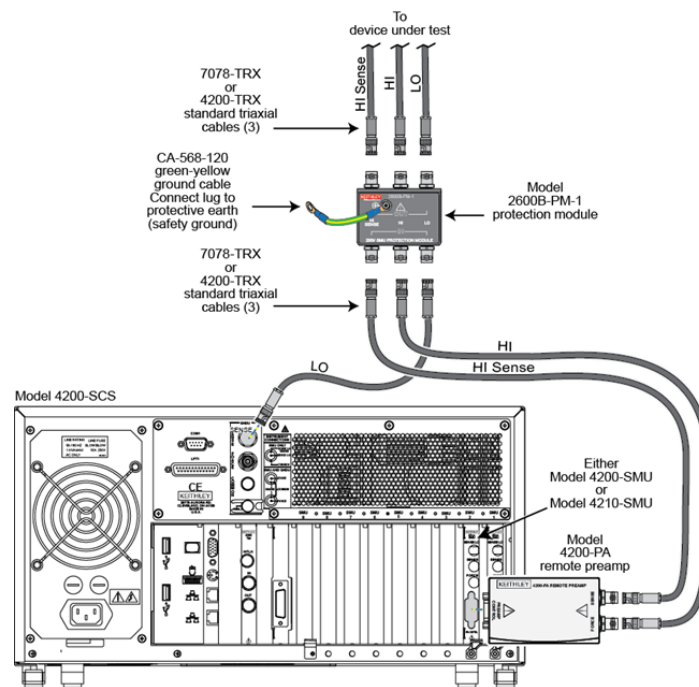
Figure 6: Model 2600B-PM-1 connections for 4200-SCS SMU with 4200-PA
