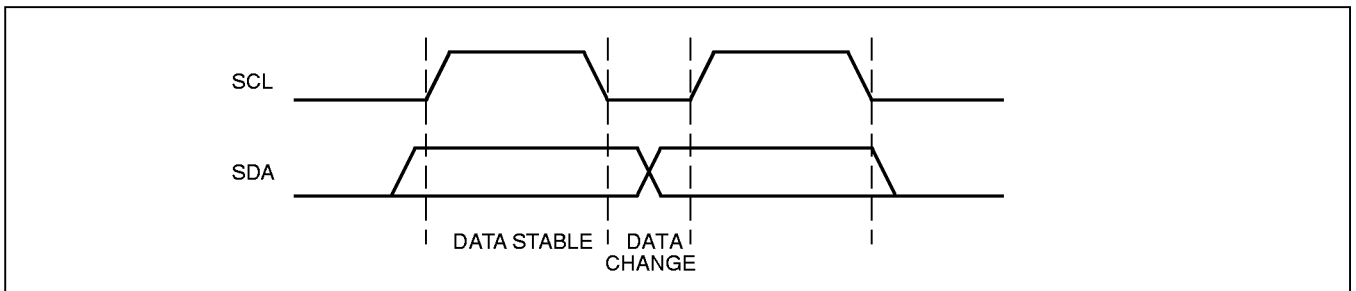
Figure 1. Data Validity
