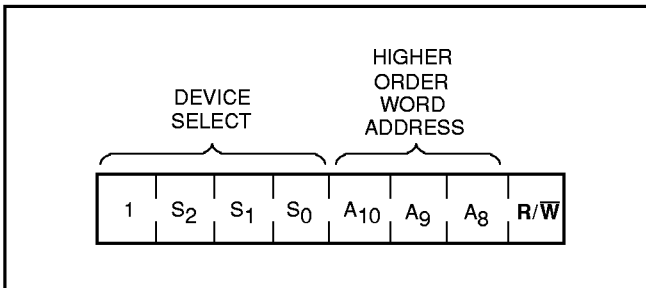
Figure 4. Slave Address
