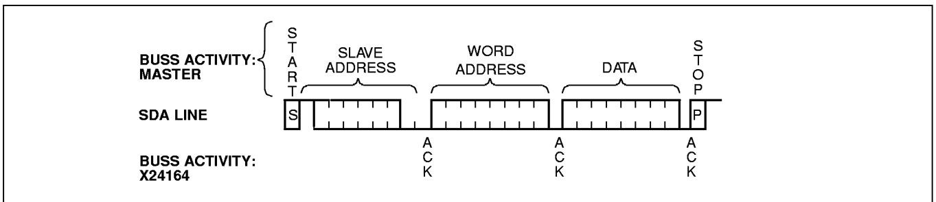
Figure 5. Byte Write
