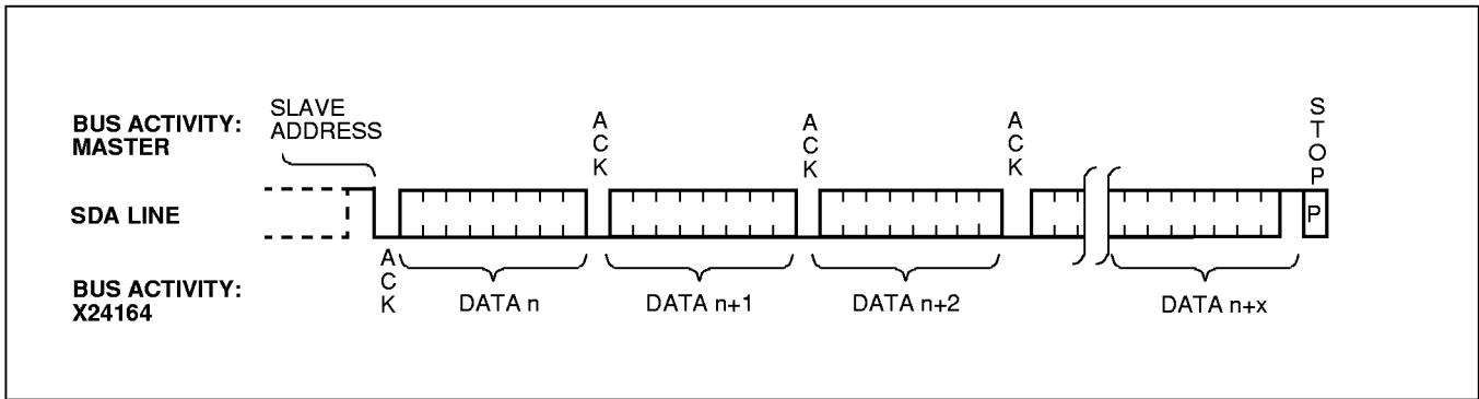
Figure 9. Sequential Read
