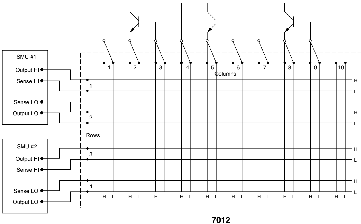
Figure 4-7 Transistor testing
