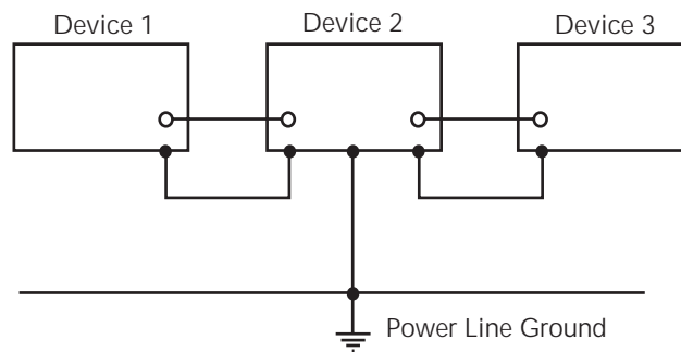
Figure 3-2 Eliminating ground loops
