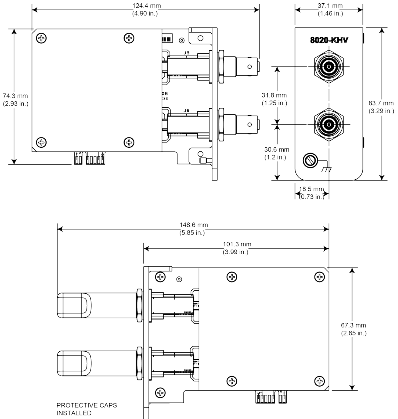
Figure 5: Model 8020-KHV dimensions
