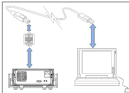
Figure 2: Communication connection
