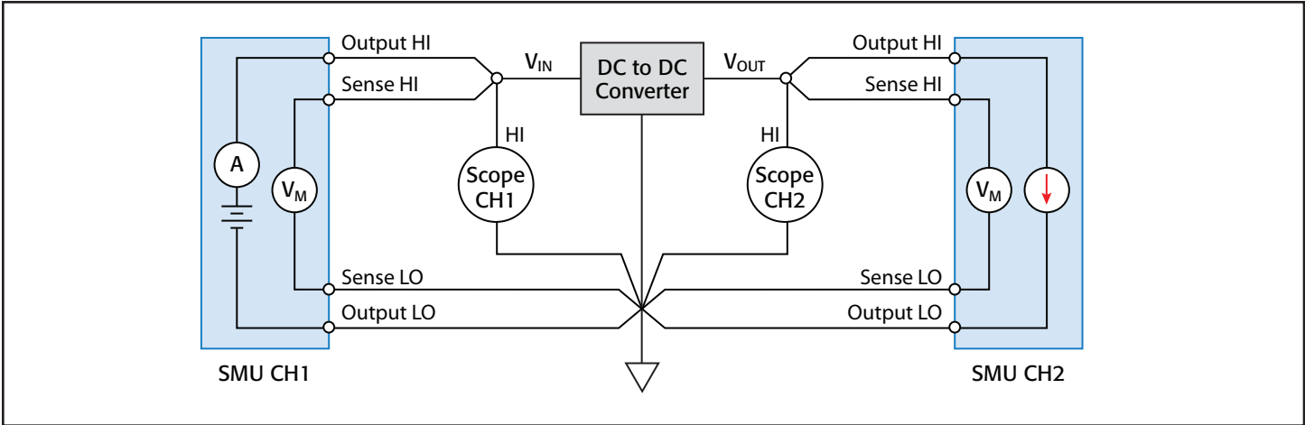
Figure 7. Testing a non-isolated DC-DC converter using both a scope and two SMUs
