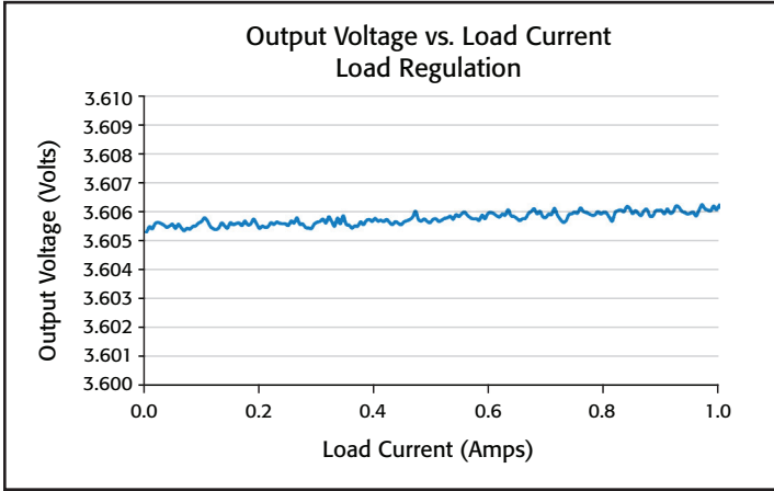
Figure 5. Plot of DC-DC converter load regulation using a two-channel Model 2612B SourceMeter SMU Instrument
