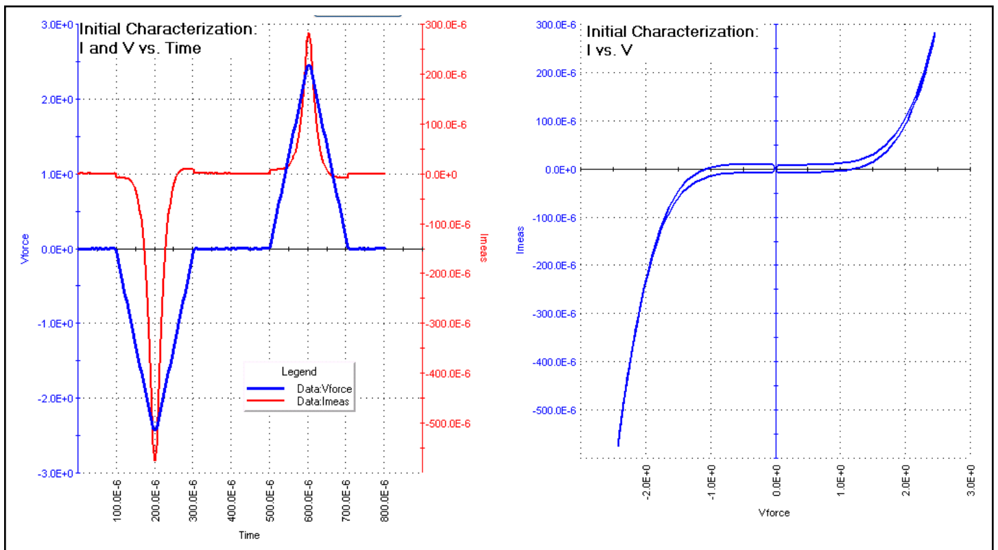
Figure 39. Characterization test of ReRAM structure.
