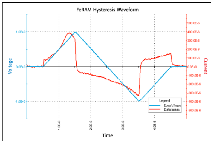
Figure 31. Hysteresis waveform generated and measured by the Model 4225-PMU with Model 4225-RPMs (user module doubleSweepSeg ). This graph shows the voltage waveform (blue) applied to the FE capacitor. The red curve shows the current flow. Figure 32 shows the typical hysteresis charge vs. voltage curve.
