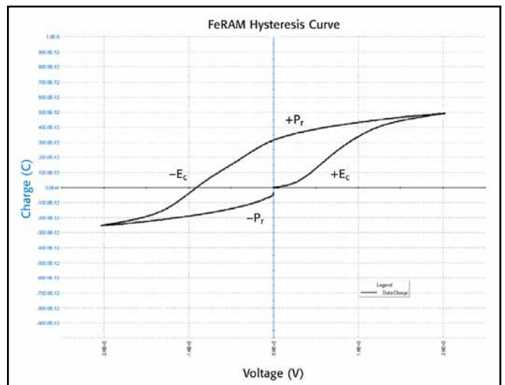
Figure 32. Hysteresis curve generated and measured by the Model 4225-PMU with Model 4225-RPMs (user module doubleSweepSeg ). This graph shows the variation in the polarity charge as the voltage across the material varies. E_c is the coercive field and P_r is the remnant polarization, which are key parameters for FeRAM performance. Proper test parameters on a good, non-leaky device should show a complete loop, with the beginning and end at 0V.
