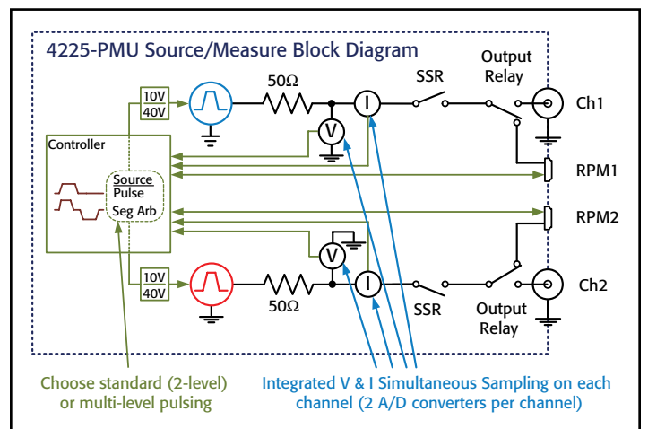
Figure 3. Model 4225-PMU Block Diagram. It is possible to use the Model 4225-PMU with two Model 4225-RPMs by using the RPM1 and RPM2 connections. The SSR shows the solid-state relay, which is useful for high impedance mode when performing program or erase on flash memory devices via Fowler-Nordheim tunneling.
