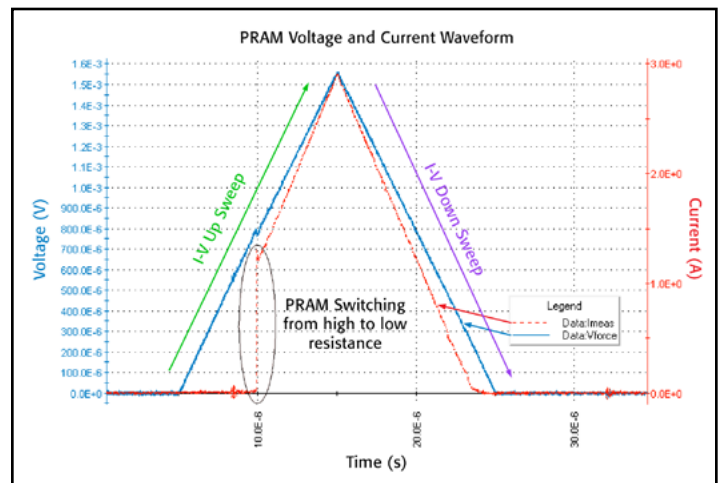
Figure 21. I-V waveform from the PRAM IV_CURVE test generated and measured by the Model 4225-PMU with Model 4225-RPMs (user module doubleSweepSeg ).
