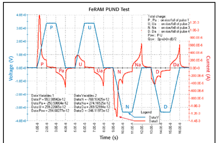
Figure 33. PUND waveforms generated and measured by the Model 4225-PMU with Model 4225-RPMs (user module pundTest ). This graph shows the applied voltage pulses and the current response. The values for P, U, N, and D are extracted from the current waveform.
