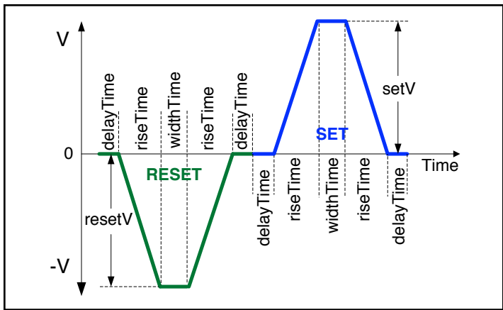
Figure 44. Pulse Waveform parameters for the stress reramEndurance.
