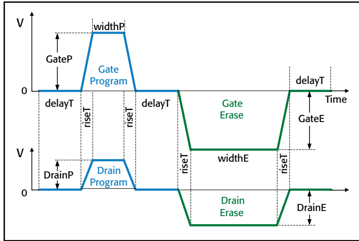
Figure 16. Waveform parameters for the flashProgramErase module.
