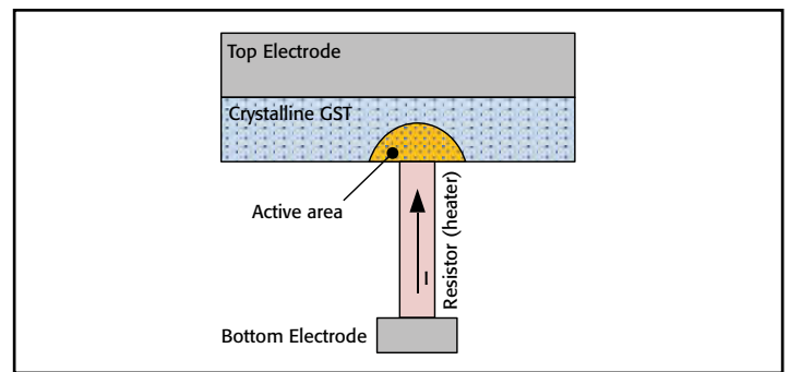
Figure 18. GST [Germanium (Ge), Antimony (Sb), and Tellurium (Te)] structure.
