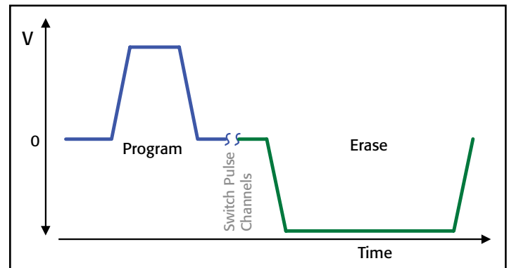
Figure 5. Flash memory Program and Erase waveform: two pulses, three levels. Traditional pulse generators can only output two level pulses, so flash testing required two pulse channels for each test pin and a time-costly switch to apply the second (negative) pulse to the test device. Note that this setup is only for one device terminal. For a typical pulsing on the gate and drain, this setup would have to be duplicated.
