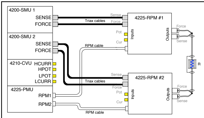
Figure 38. Connection to the 2 terminal ReRAM device.
