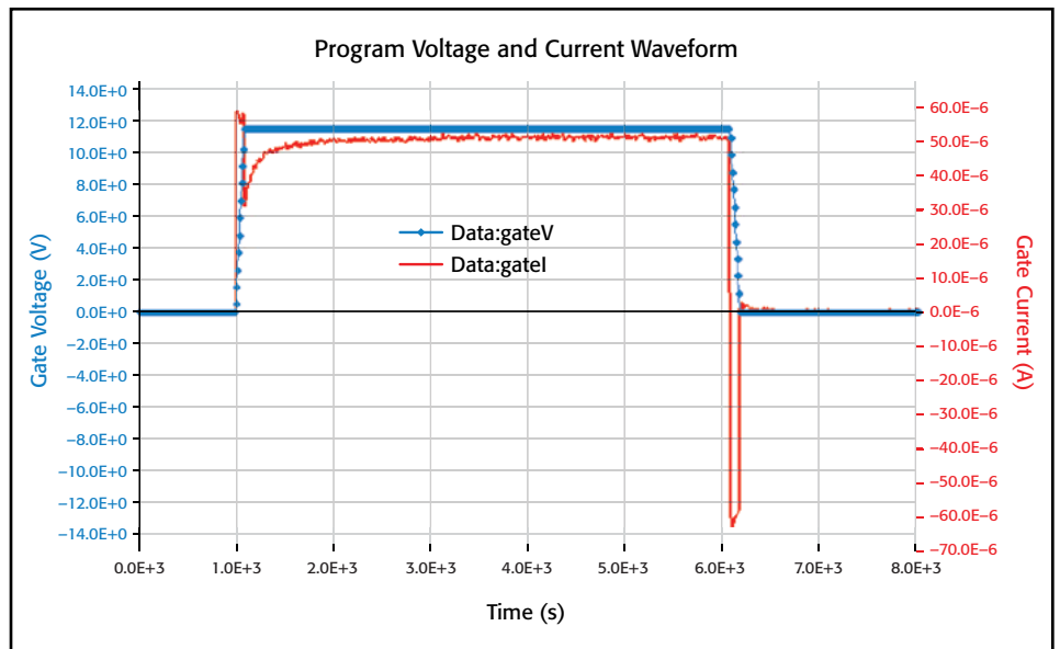
Figure 13. Pulse current and voltage waveforms for a Program pulse on a NAND cell using a Model 4225-PMU with Model 4225-RPMs. Note the capacitive charging and discharging current during the pulse transitions (see “Optimizing Measurements” for an explanation). This graph is from the Flash Program test (user module flashProgramErase ).
