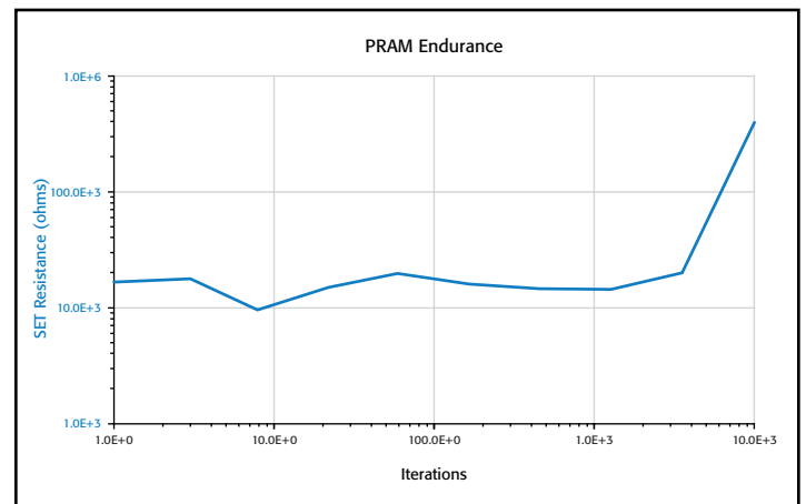
Figure 26. PRAM endurance curve generated and measured by the Model 4225-PMU with Model 4225-RPMs (user module pramEndurance ).
