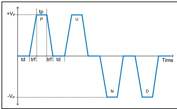
Figure 36. Pulse waveform parameters for pundTest .
