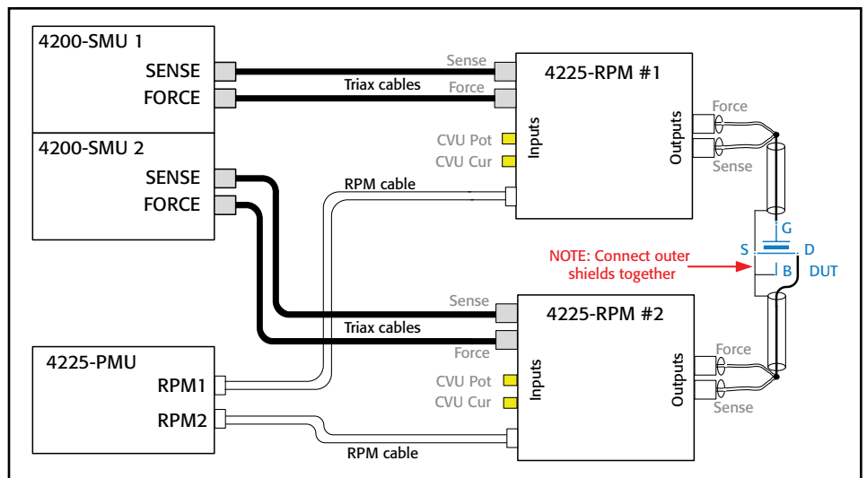
Figure 12. Connection to four-terminal floating gate flash device.
