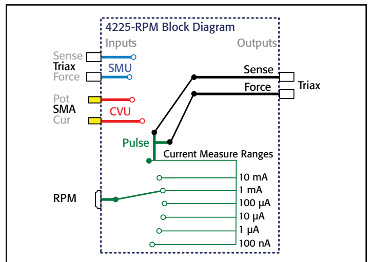
Figure 4. Model 4225-RPM Block Diagram. The Model 4225-RPM is both a current pre-amplifier for high speed current measure (in Pulse mode) and a switch for use in choosing between Pulse I-V, SMU, or C-V measurement modes for other instruments in the Model 4200-SCS chassis.
