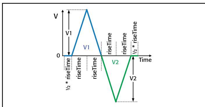
Figure 27. The multi-pulse waveform of doubleSweep .
