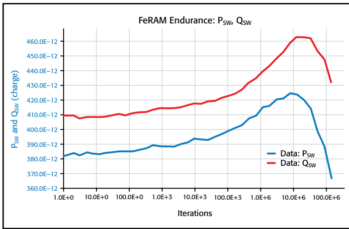
Figure 34. FeRAM endurance, showing the degradation in P_{SW} and Q_{SW} (user module pundEndurance ). Some FeRAM endurance curves only show Q_{SW} . This data was taken by the Model 4225-PMU with Model 4225-RPMs.
