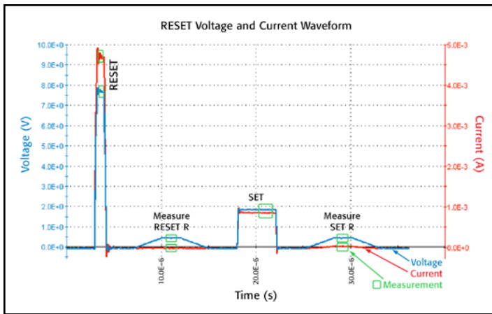
Figure 23. R-I RESET-Measure-SET-Measure waveform generated and measured by the Model 4225-PMU with Model 4225-RPMs (user module pramSweep ). This graph shows the voltage (blue, left y-axis) and current (red, right y-axis) waveforms. There are four pulses within this waveform. The first pulse is the RESET pulse, which resets the PRAM material, putting it into a high resistance, amorphous state. The second pulse measures the resistance of the RESET state. The third pulse is the SET pulse, which will put the material into a low resistance, crystalline state. The fourth and last pulse measures the resistance of the material in the SET state. Figure 24 is an R-I curve that results from sweeping the SET pulse height and plotting the results in the R-I curve.
