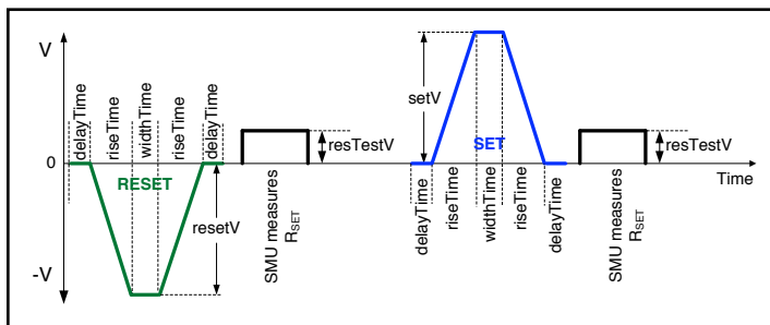
Figure 43. Pulse waveform with measure for reramSweep and reramEndurance .
