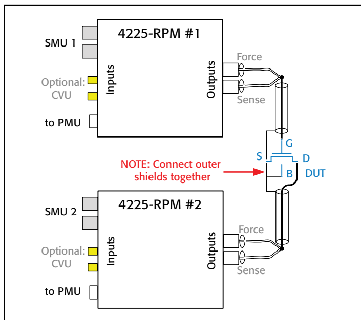
Figure 8. Connection to four-terminal test device with two Model 4225-RPMs.
