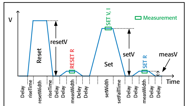
Figure 28. PRAM waveform definition.
