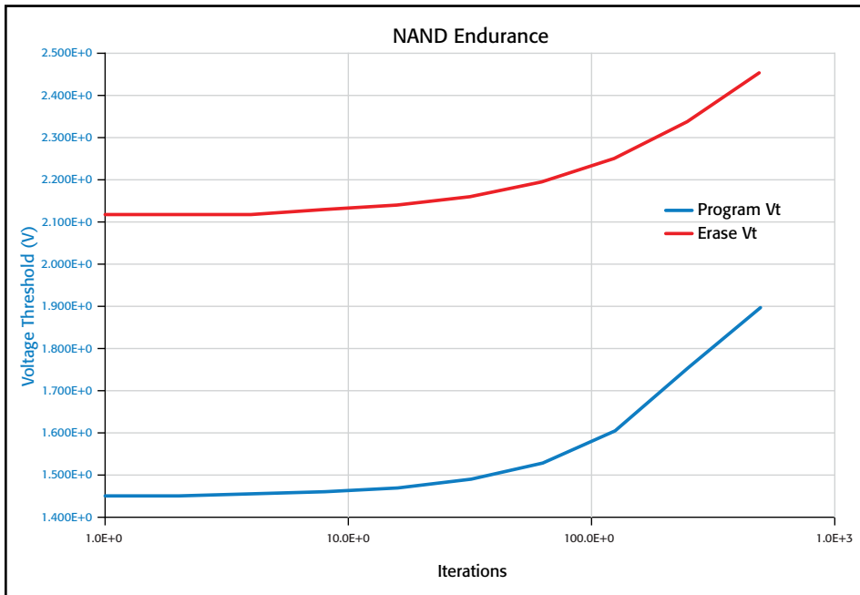
Figure 15. NAND flash endurance results from the Flash UTM Endurance test (user module flashEndurance ).
