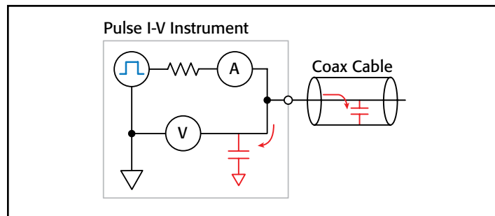
Figure 48. Block diagram of pulse I-V instrument showing the capacitive charging current during pulse transitions.
