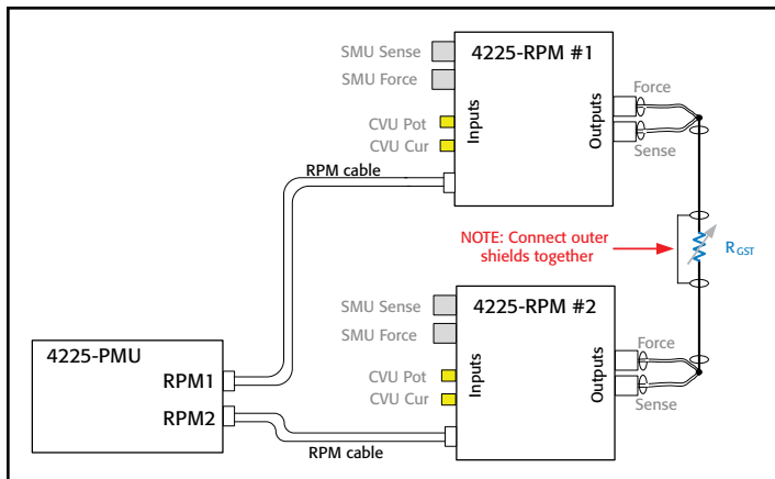
Figure 19. Connection diagram for PRAM tests. Note that the PRAM tests included with NVM_Examples do not use the SMUs or CVU.
