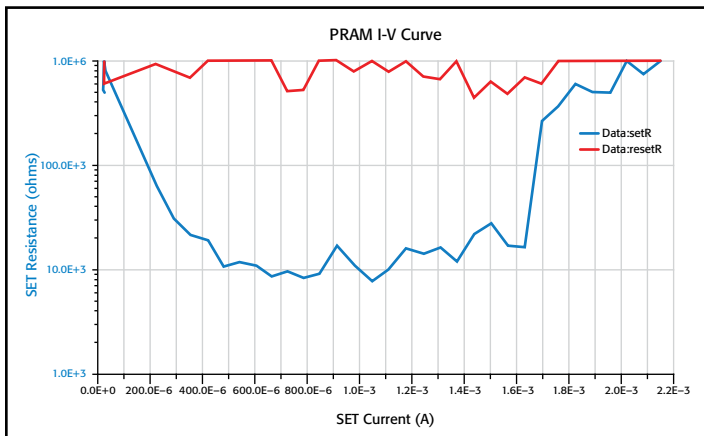
Figure 24. R-I curve shows the resistance variation of the SET state resistance generated and measured by the Model 4225-PMU with Model 4225-RPMs (user module pramSweep ). This test uses the data captured from the tops of the pulses shown in Figure 23 .
