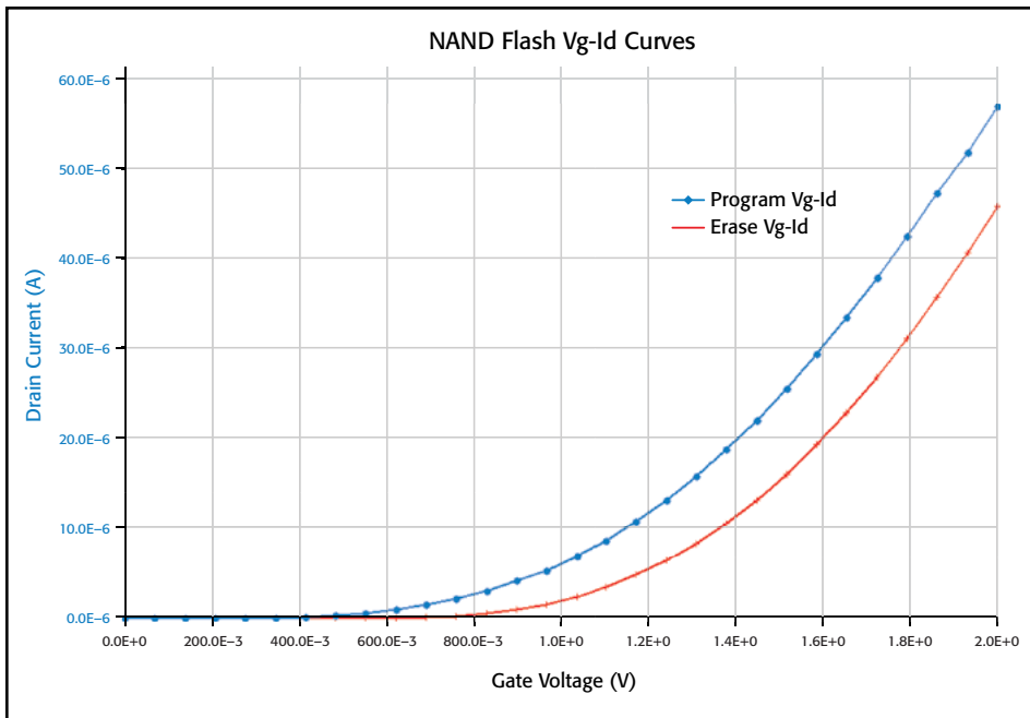
Figure 14. V_T sweeps for a programmed and erased cell taken with SMUs, from the V_T Erased UTM (user module vt_ext ). In this graph, the difference in the V_T after program and after erase is about 180mV.
