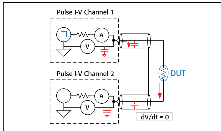
Figure 50. Block diagram of two pulse I-V channels connected to a two-terminal device.
