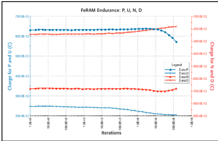
Figure 35. FeRAM endurance, showing the degradation in P, U, N, and D values (user module pundEndurance ). This data is used to create the data in Figure 34. This data was taken by the Model 4225-PMU with Model 4225-RPMs.
