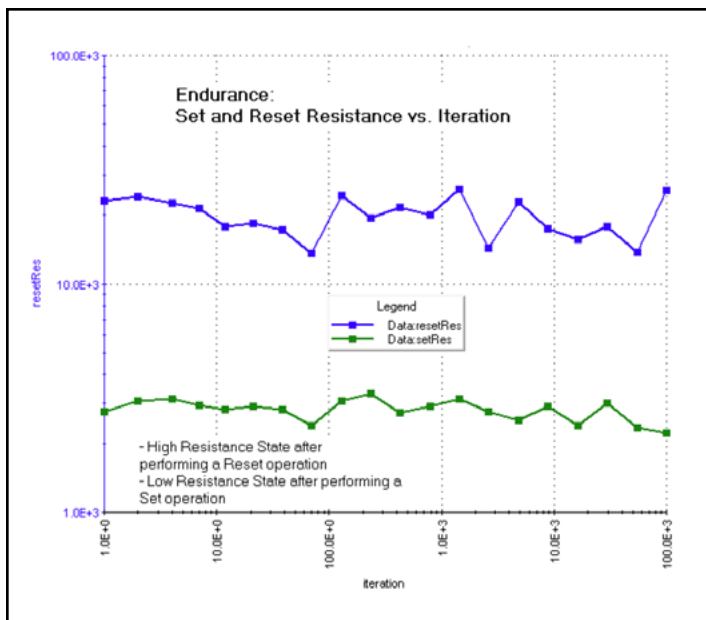
Figure 42. ReRAM endurance test.
