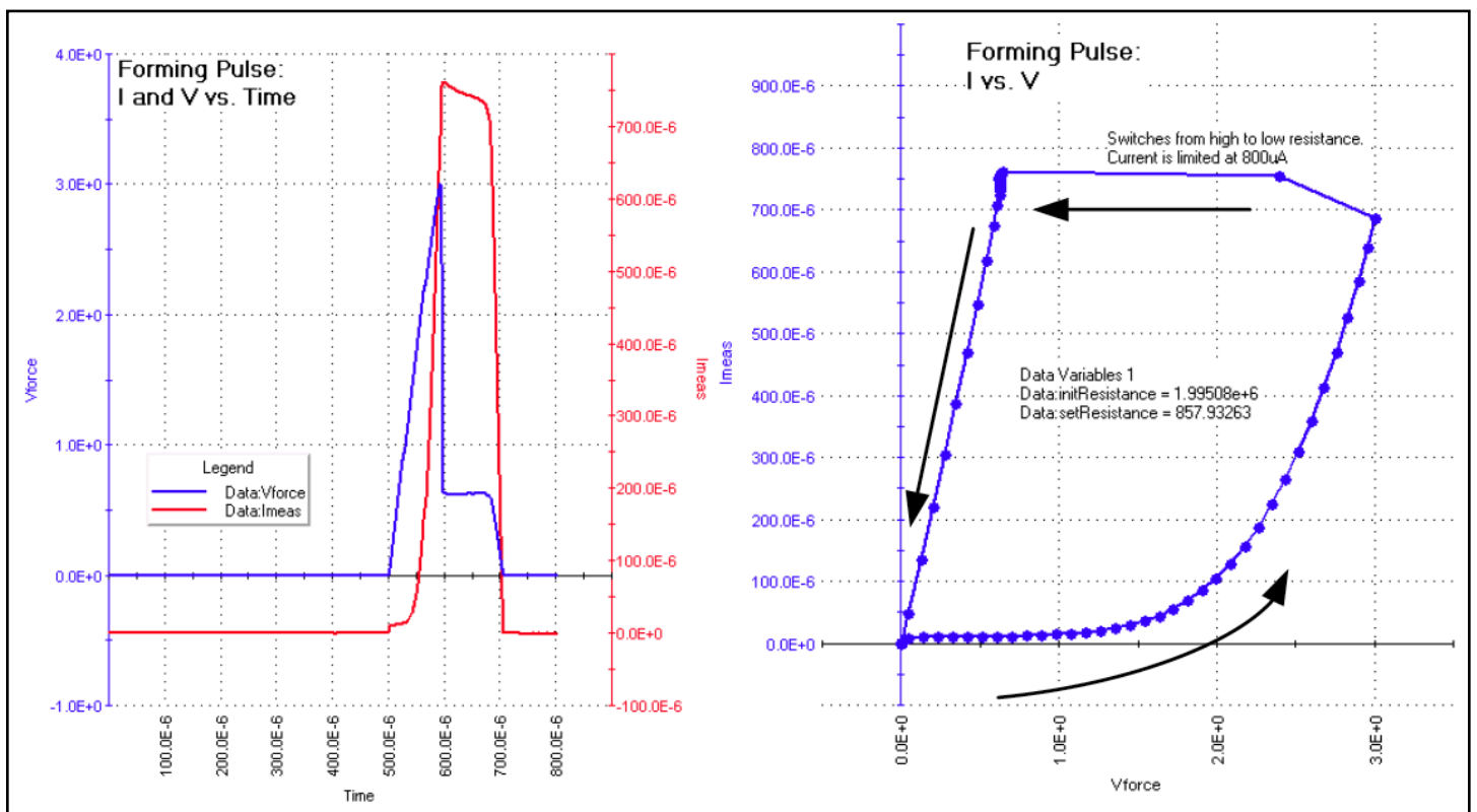
Figure 40. ReRAM forming.
