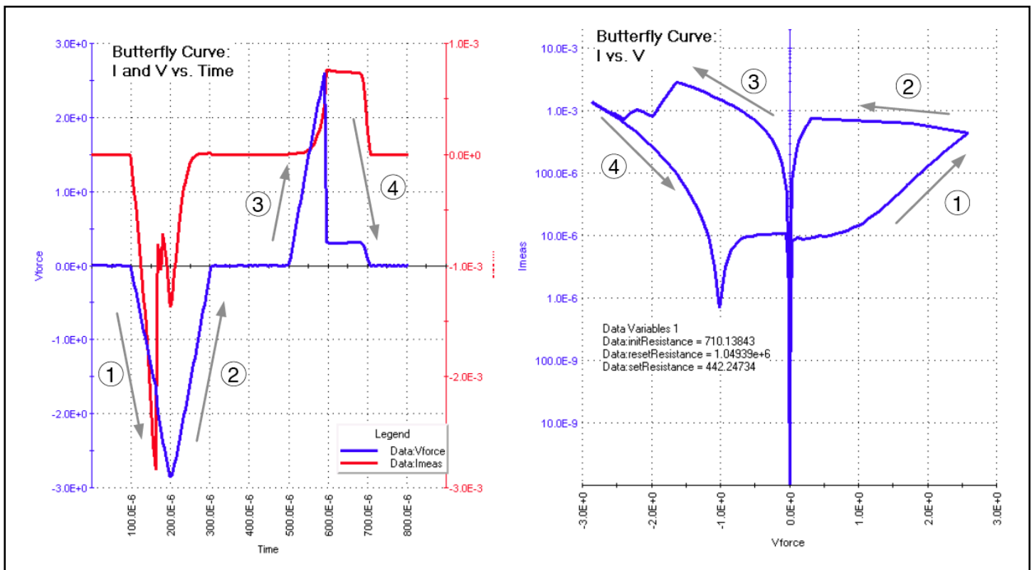
Figure 41. ReRAM "Butterfly" curve.
