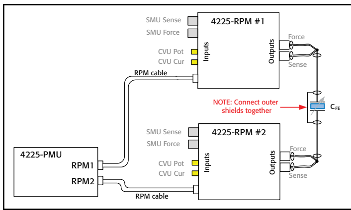
Figure 30. Connection for FeRAM tests. Note that the FeRAM tests included with NVM_Examples do not use the SMUs or CVU.
