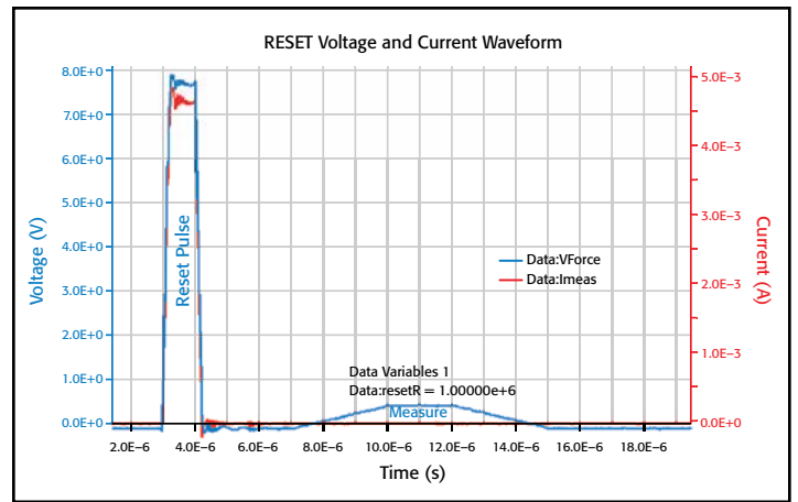
Figure 20. PRAM RESET waveform generated and measured by the Model 4225-PMU with Model 4225-RPMs (user module pramSweep ).
