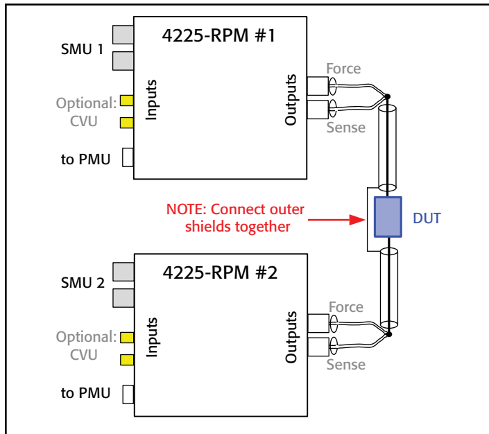
Figure 7. Connection to two-terminal test device.
