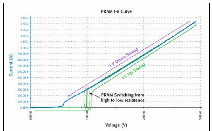
Figure 22. I-V curve from the PRAM IV_CURVE test generated and measured by the Model 4225-PMU with Model 4225-RPMs. This test uses the same data shown in Figure 21, but the curve plots I vs. V (user module doubleSweepSeg ).
