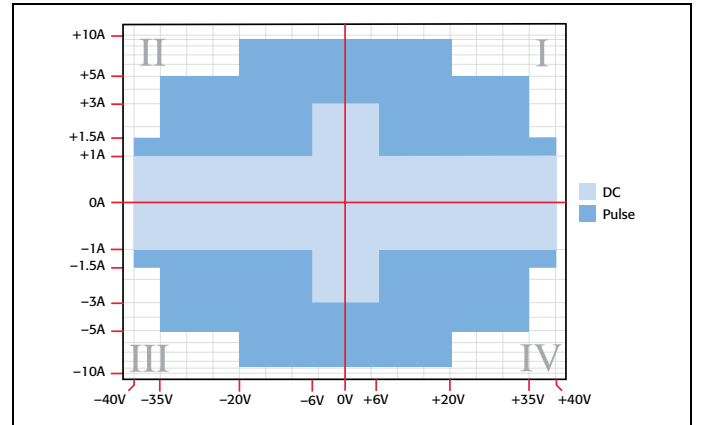
Models 2601B, 2602B, and 2604B I-V capability
