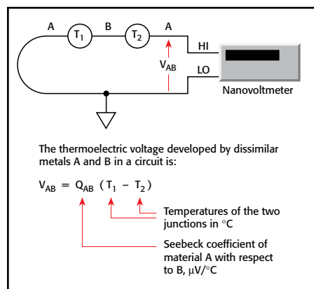
Figure 1. Thermoelectric EMFs
