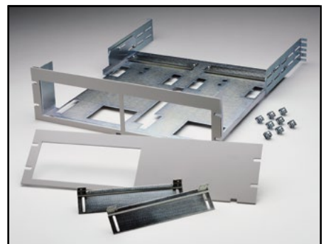
Model 4288-5 Fixed Rack Mount Kit: The single- and dual-instrument front panels included enable rack mounting of either one or two 3½-inch instruments. Height: 132mm (5¼ in). Depth: 457mm(18 in).
