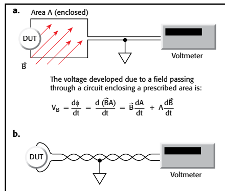
Figure 3. Minimizing interference from magnetic fields with twisted leads
