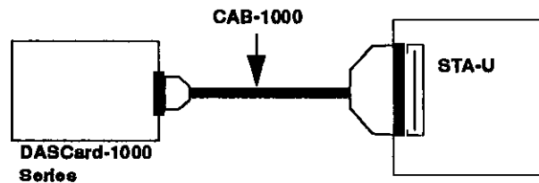
Figure 1. Connecting the DASCARD-1000 Series Card to an STA-U
