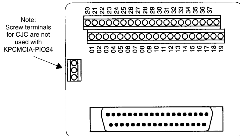
Figure 6-4 Panel layout of STP-37 and STP-37/C
