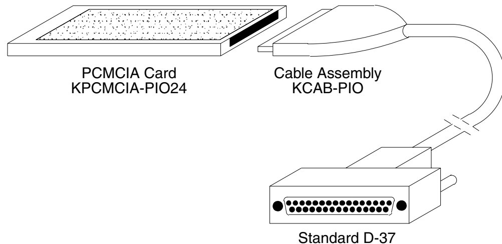
Figure 1-1 System configuration
