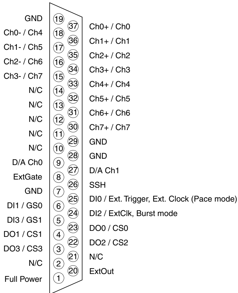
Figure 6-1 KPCMCIA-12AIAO/16AIAO PC card D-37 output connector, KCAB-AIAO
