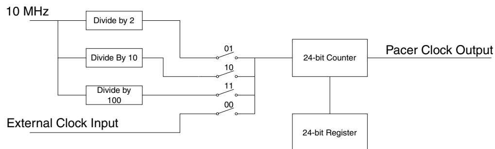
Figure 5-1 Pacer clock block diagram
