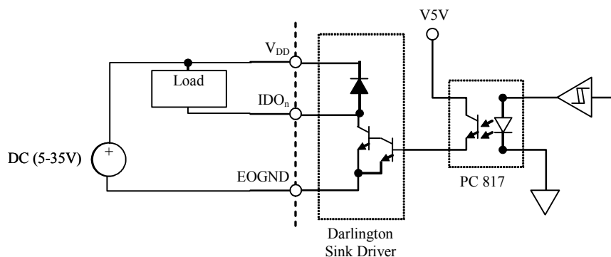
Figure 3-2 Isolated digital output circuits wiring diagram
