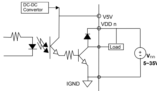
Figure 3-3 Common Ground Connection
