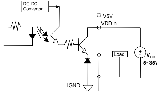
Figure 3-4 Common Power Connection
