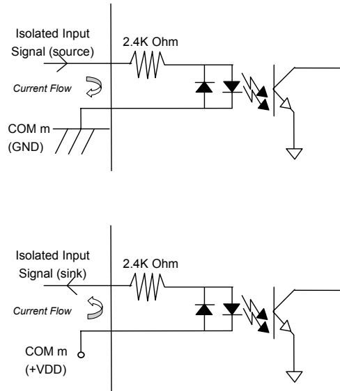
Figure 3-1 Isolated isolated input connections
