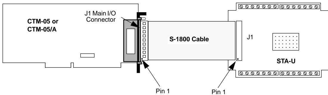
Figure 1. Connecting the CTM-05 or CTM-05/A Board to an STA-U
