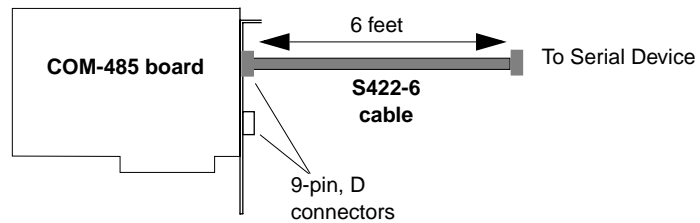
Figure 1. Connecting the COM-485 Board
