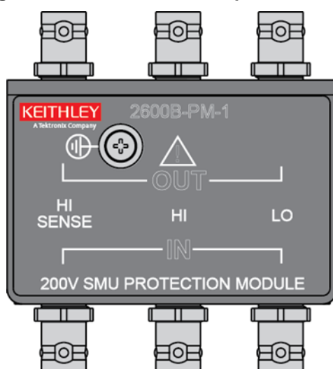
Figure 1: Model 2600B-PM-1 protection module
