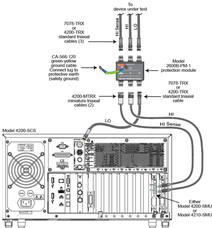
Figure 6: Model 2600B-PM-1 connections for Model 4200-SCS SMU
