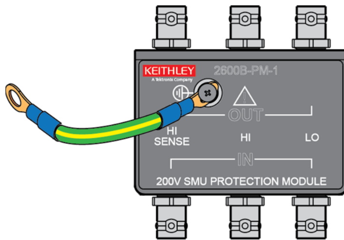
Figure 2: Model 2600B-PM-1 grounding
