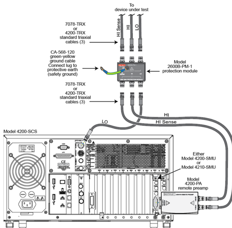
Figure 5: Model 2600B-PM-1 connections for 4200-SCS SMU with 4200-PA
