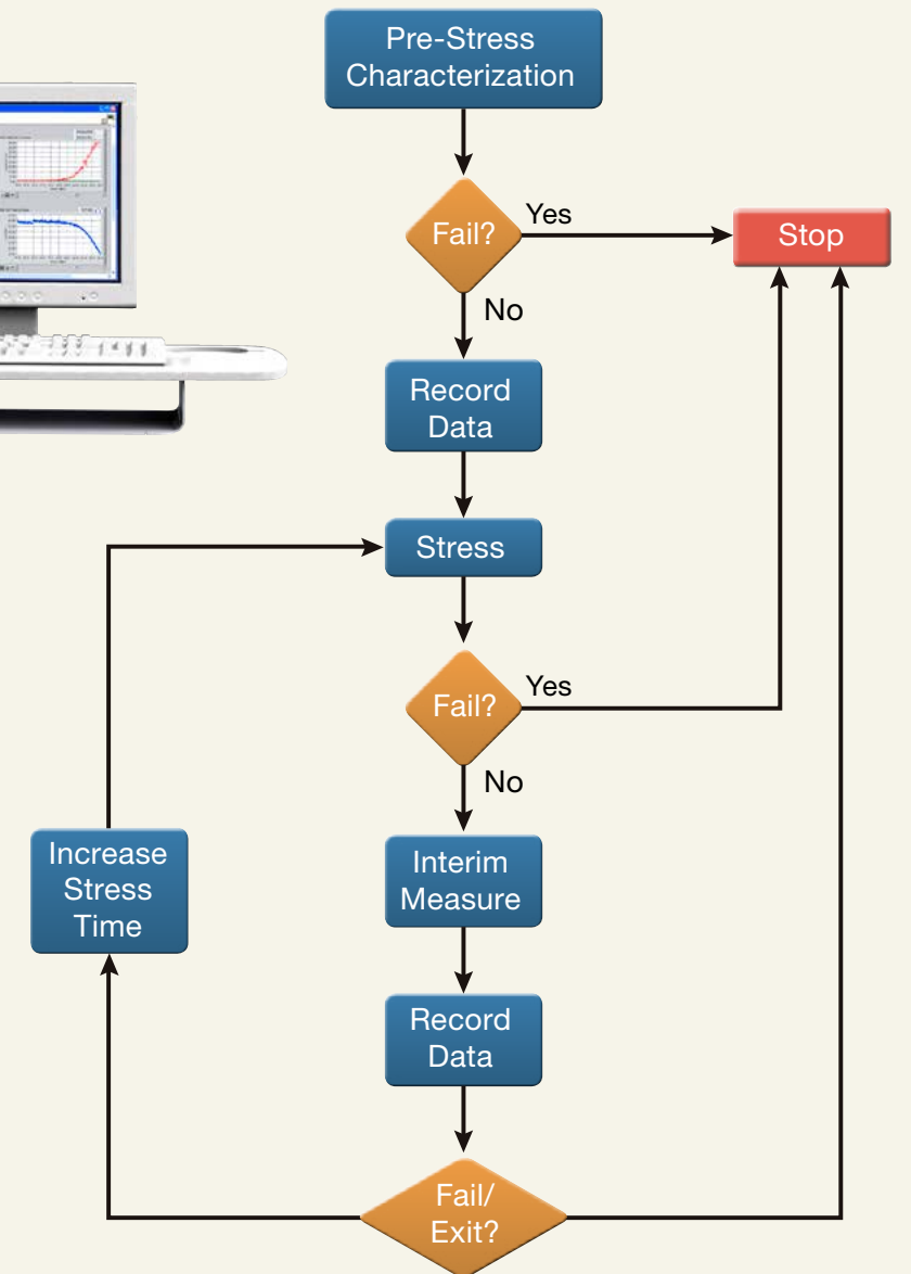
Process flow for HCI/NBTI/constant current EM tests.
