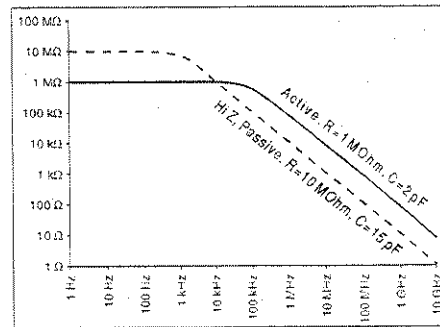
Probe Impedance versus Frequency
