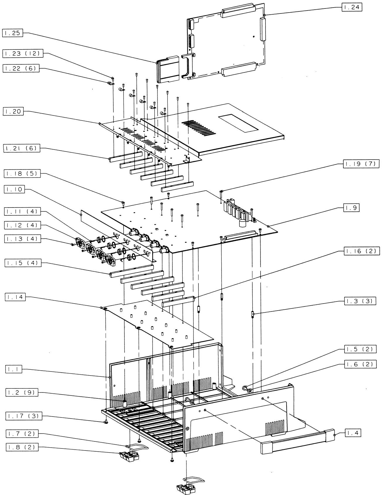
FIGURE 7.2: 9320 LOWER COVER EXPLODED VIEW
