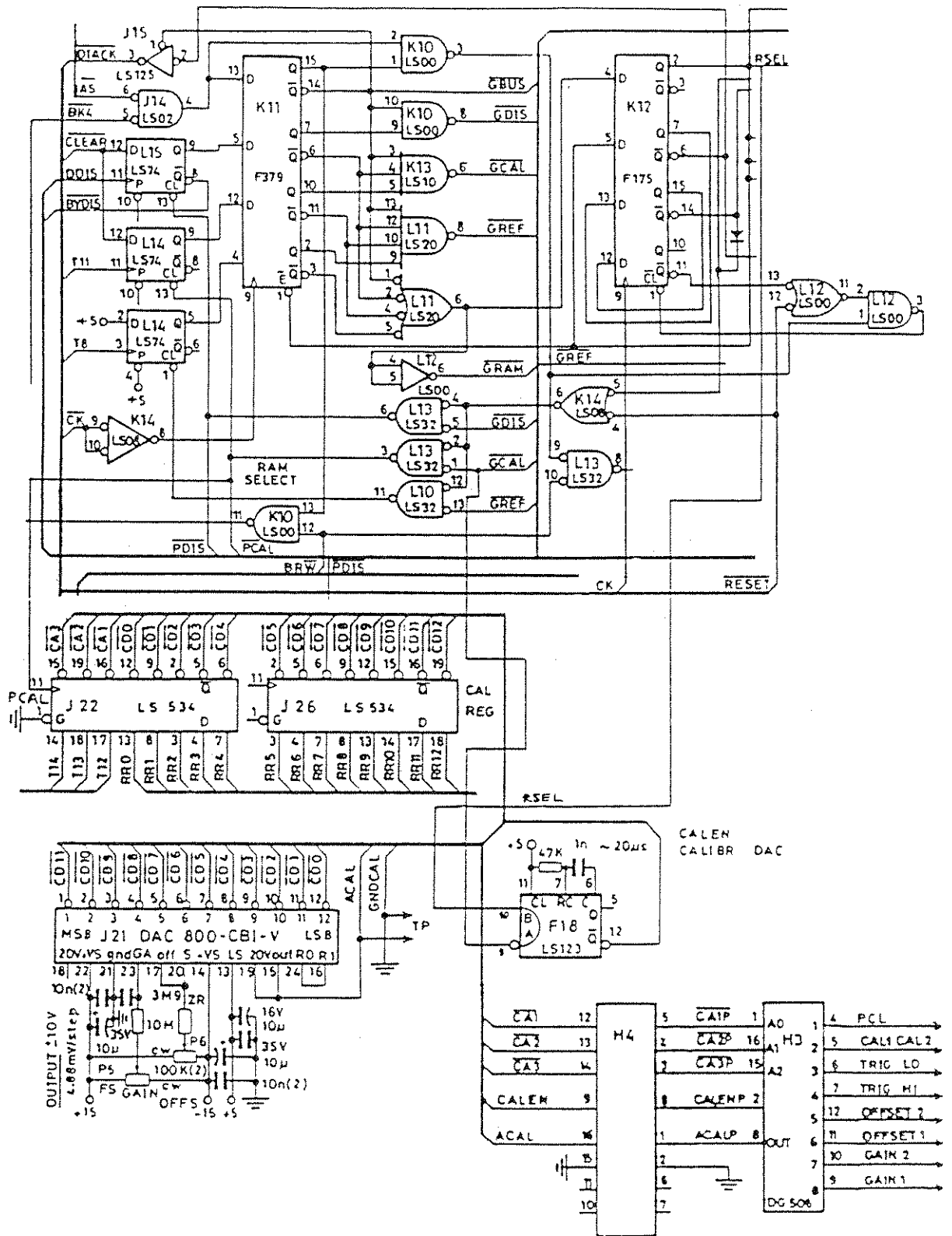
CALIBRATION CONTROLLER
