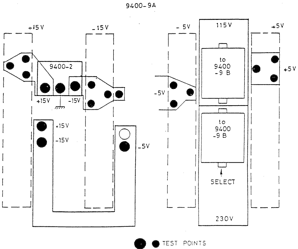
SETTING THE 115 V/220 V CONNECTION
