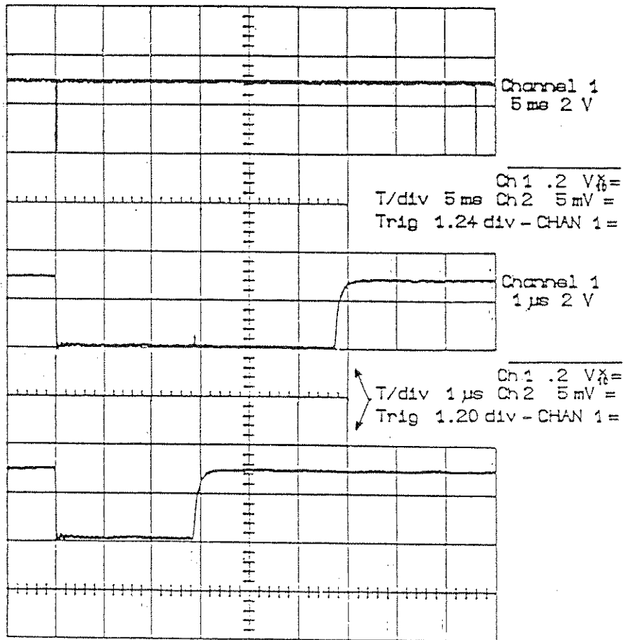
SIGNALS ON FDO IN A TYPICAL CASE
