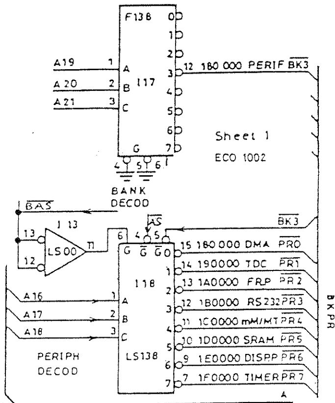
PERIPHERAL DECODER
