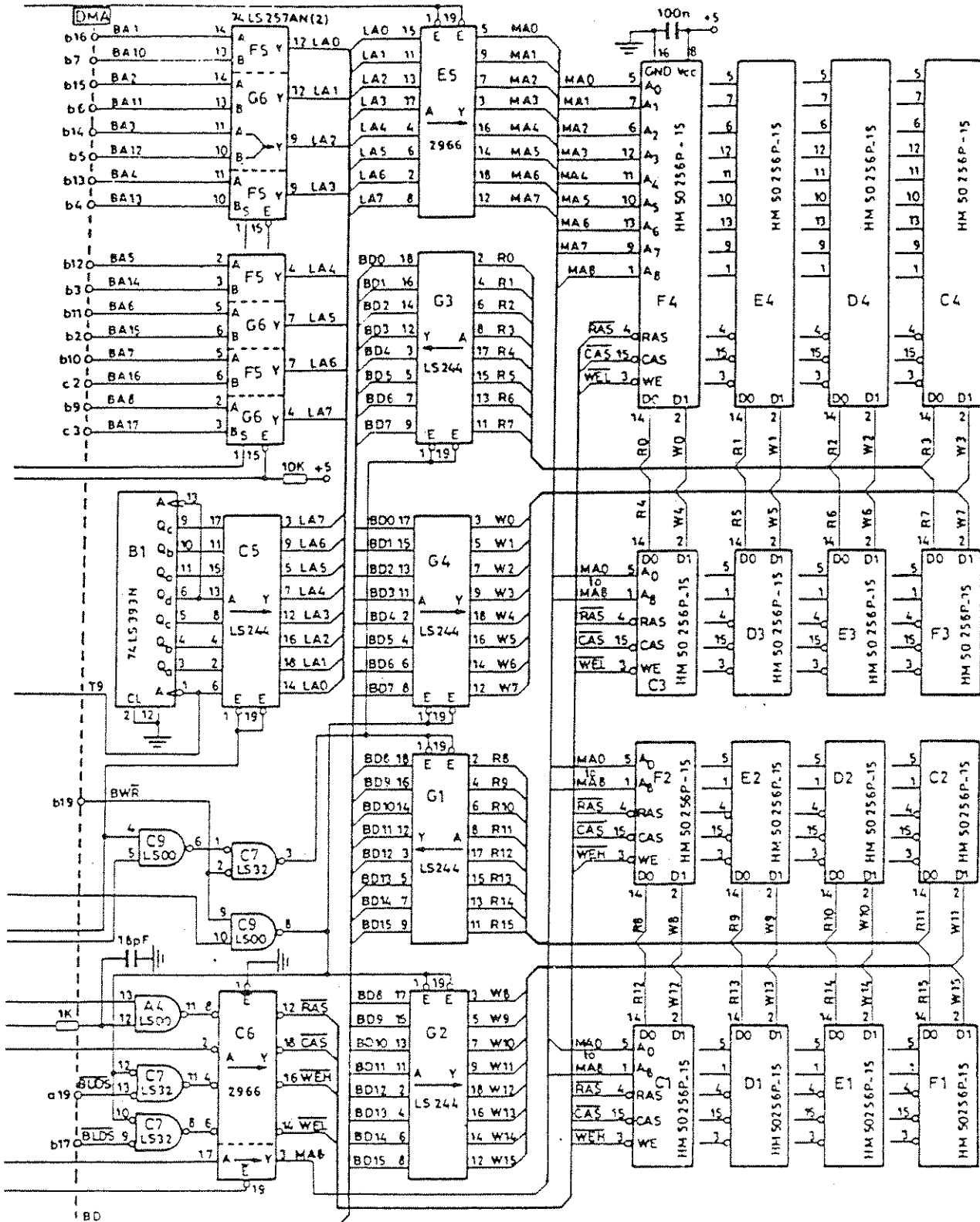
LeCroy 9401-2/1-S1 and 9401-2/2-S1 Sheet 3 of 4 ECO:1002
