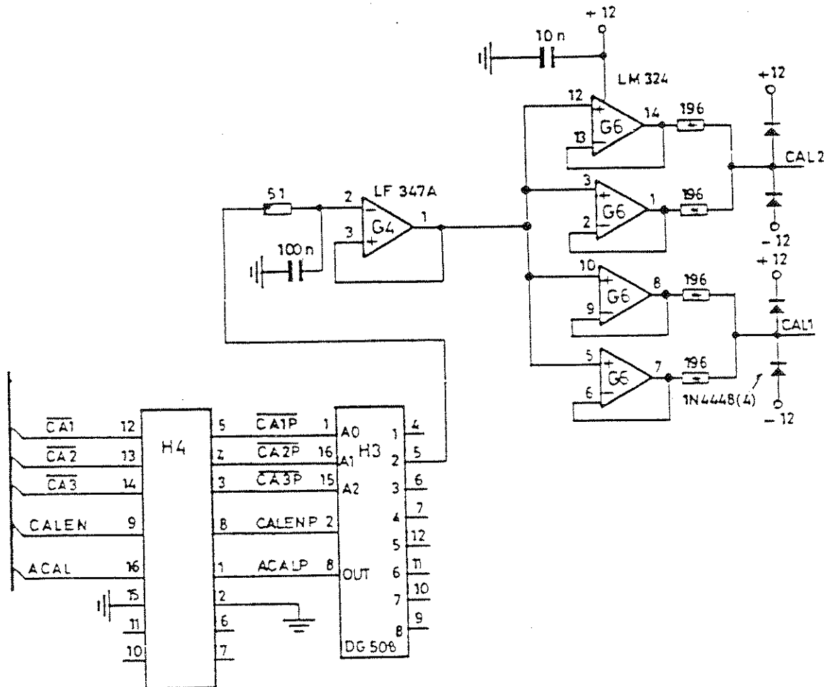
CALIBRATION SYSTEM
