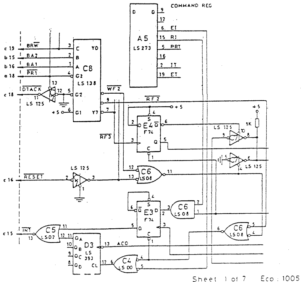
INTERRUPT CONTROLLER
